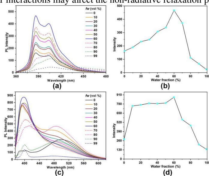
Fig. 5. (a), (c) PL spectra of 3a and 3f in THF/water mixtures with different water fractions ( f_w ), respectively. (b), (d) Plot of PL intensity at different fractions (0–99 vol%) for 3a and 3f .
