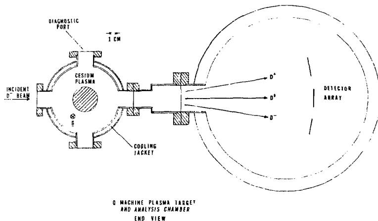
Fig. 8. Experimental arrangement for determination of \sigma_{D^0} and \sigma_{D^+} in a cesium plasma target.
