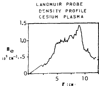
Fig. 9. Electron density (derived from Langmuir probes) vs position in the cesium plasma target.
