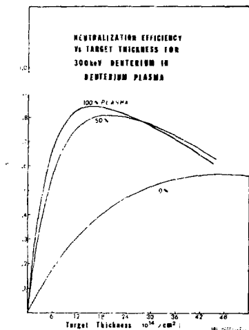
Fig. 3. Neutralization efficiency versus total (electrons and ions and neutrals) target thickness for 300 keV deuterium in a deuterium plasma of various degrees of ionization.
