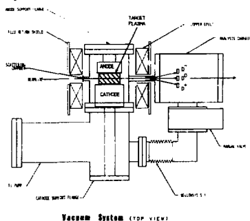
Fig. 6. Experimental arrangement for determination of n_{\max} in a hydrogen plasma target.
