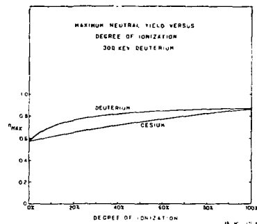
Fig. 5. Maximum neutralization efficiency versus degree of ionization for deuterium and cesium plasmas.
