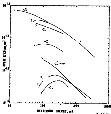
Fig. 2. Cross sections relevant to cesium plasma neutralizers. Curve 1, Ref. 5. ( \sigma_{CS^+} is taken to be equal \sigma_{H^+} for the purpose of the computations); 2, Refs. 6, 7; 3, Ref. 15; 4, Ref. 15; 5, Ref. 16; 6, Ref. 13; 7, Ref. 14.
