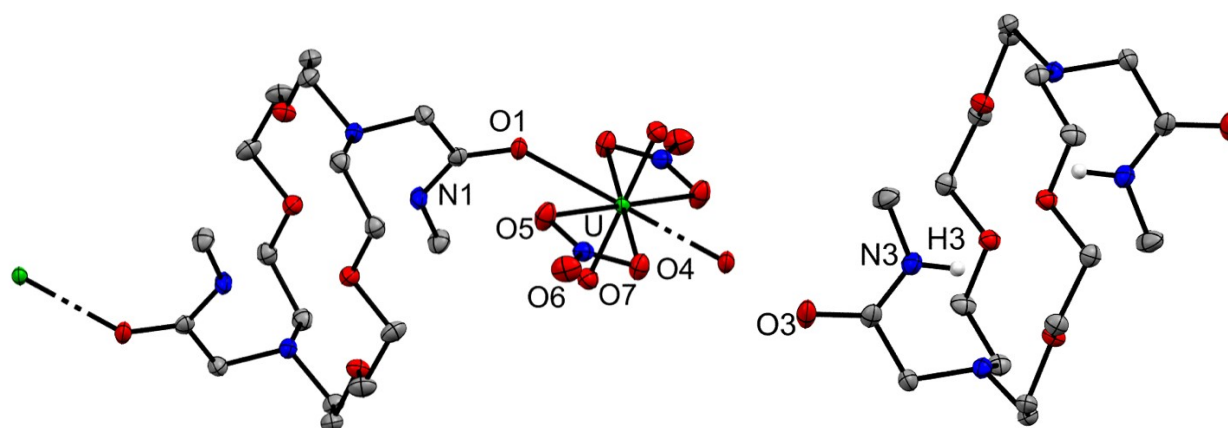
Figure 3. Solid-state molecular structures of 3 (left) and BAM ·5H 2 O (right) shown with 50% probability ellipsoids and hydrogen atoms are omitted for clarity. Selected bond lengths (Å) and angles (°): 3 : O1-U = 2.378(1), O5-U = 2.510(1), O4-U = 2.544(2), O7-U = 1.763(1), O7-U-O7* = 180. BAM ·5H 2 O: N2-N3 = 2.6736(15).
