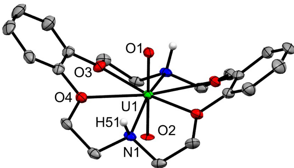
Figure 1. Solid-state molecular structure of 1 \cdot 2\text{MeCN} \cdot \text{Et}_2\text{O} shown with 50% probability ellipsoids. Solvate molecules, triflate counterions, and hydrogen atoms are omitted for clarity. Selected bond lengths (Å) and angles ( ^\circ ): \text{U1}-\text{O1} = 1.768(4) , \text{U1}-\text{O2} = 1.765(4) , \text{U1}-\text{O3}
