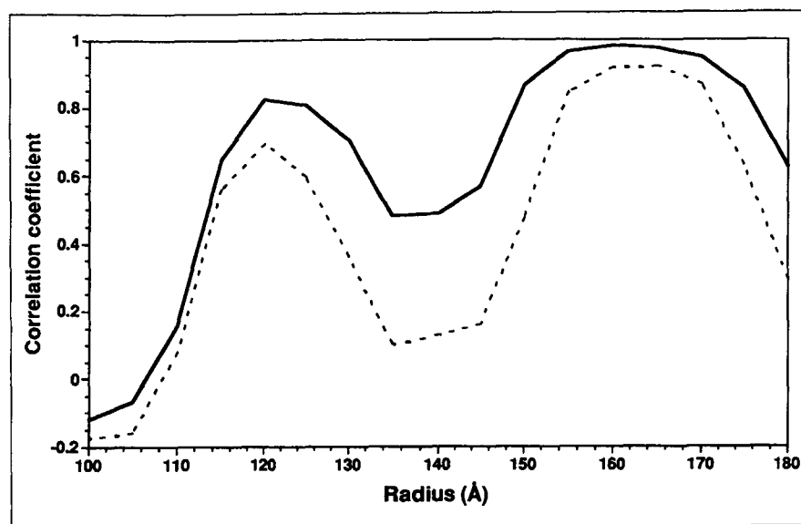
Fig. 10. Plot of correlation coefficients as a function of virus radius, comparing the X-ray model with cryoEM reconstructions before (dashed line) and after (solid line) corrections were made to reduce the effects of the microscope contrast transfer function. The plots clearly demonstrate marked improvement in the data within the capsid shell after compensation for the defocus effects were included.
