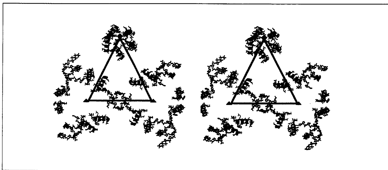
Fig. 2. Stereoview of the \gamma -peptides and ordered RNA segments of the FHV particle structure. The triangle represents the border of the icosahedral asymmetric unit containing A, B and C in the T=3 particle in Fig. 1. Blue helices are associated with the A subunits ( \gamma_A ), red with the B subunits ( \gamma_B ), and green with the C subunits ( \gamma_C ). Quasi six-fold axes are shown as red triangles, the five-fold axes as a red pentagon. Duplex RNA is represented as ball-and-stick models.
