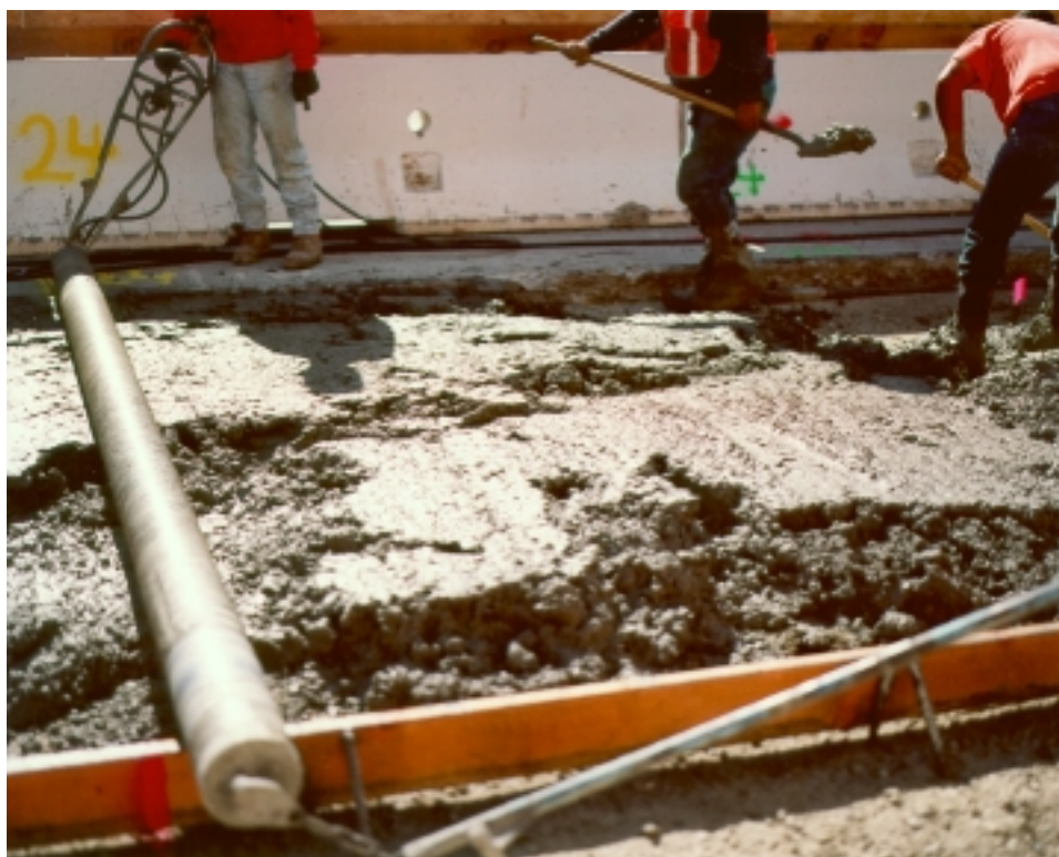
Figure 8.2. Unworkable Mix on South Tangent.
