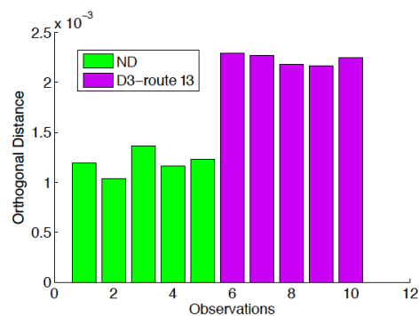
Figure 15. Damage detection using OD, case study 2, 400KHz, route 1 → 3, damage 3.
