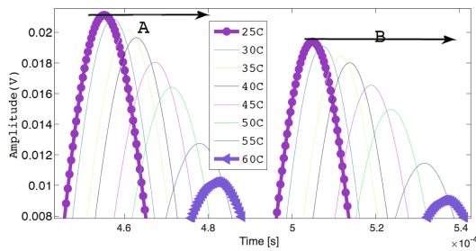
Figure 19. Propagated wave at different temperatures: Case study 1
