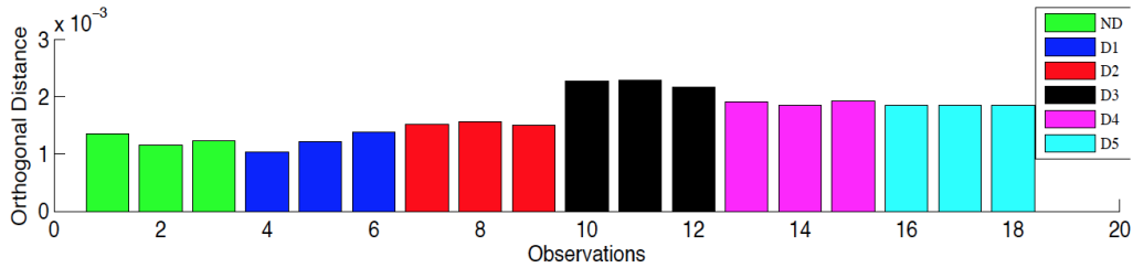
Figure 18. Damage detection using OD, case study 2, 400KHz, route 3 \rightarrow 1, all damages.
