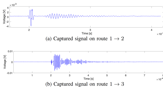
Figure 5. Example of the signal captured in two routes.
