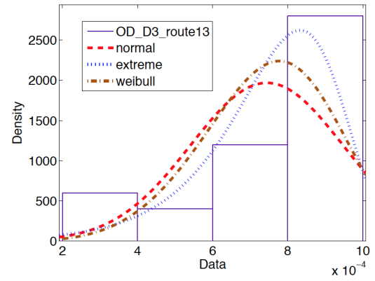
Figure 10. OD distribution, case study 1, D3, route 1 \rightarrow 3
