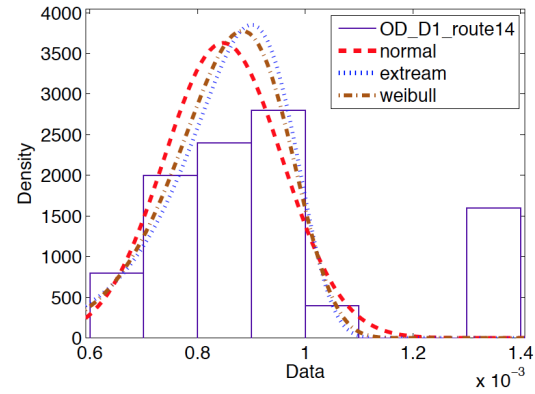
Figure 12. OD distribution, case study 1, D1, route 1 \rightarrow 4
