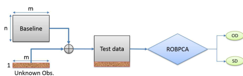
Figure 3. Damage detection methodology using OD.
