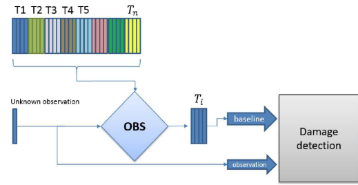
Figure 2. Schematic of OBS temperature compensation.
