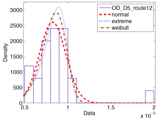
Figure 8. OD distribution, case study 1, D5, route 1 \rightarrow 2
