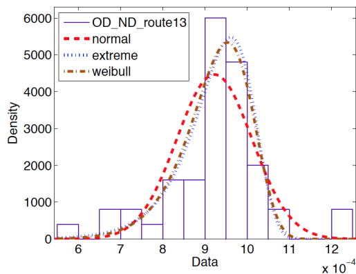
Figure 9. OD distribution, case study 1, healthy, route 1 \rightarrow 3
