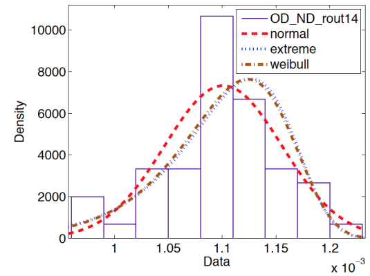
Figure 11. OD distribution, case study 1, healthy, route 1 \rightarrow 4
