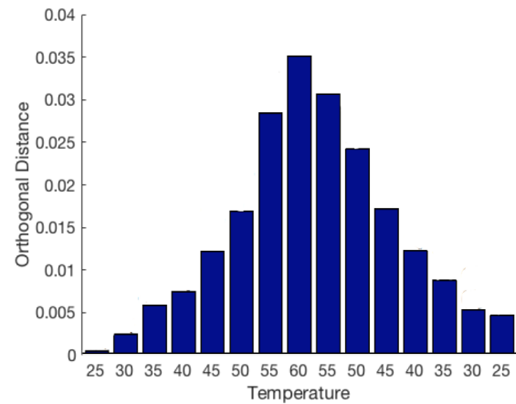
Figure 21. Temperature effect on OD, case study 1, route 1 \rightarrow 2
