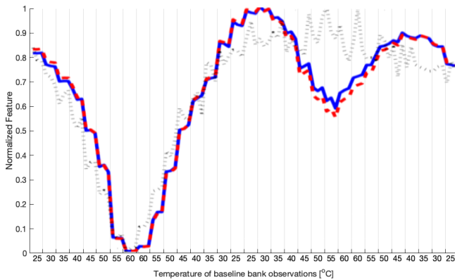
Figure 24. Differential features comparison: ND 60°C in case study 1.
