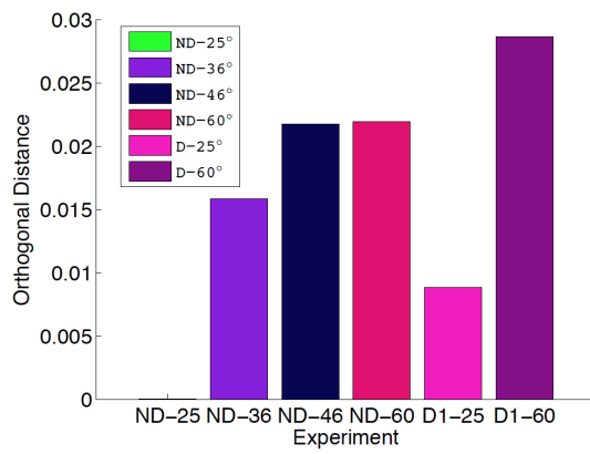
Figure 23. Temperature effect on damage detection using OD: Case study 2, route 1 → 4
