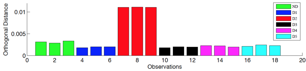
Figure 17. Damage detection using OD, case study 2, 400KHz, route 2 \rightarrow 1, all damages.
