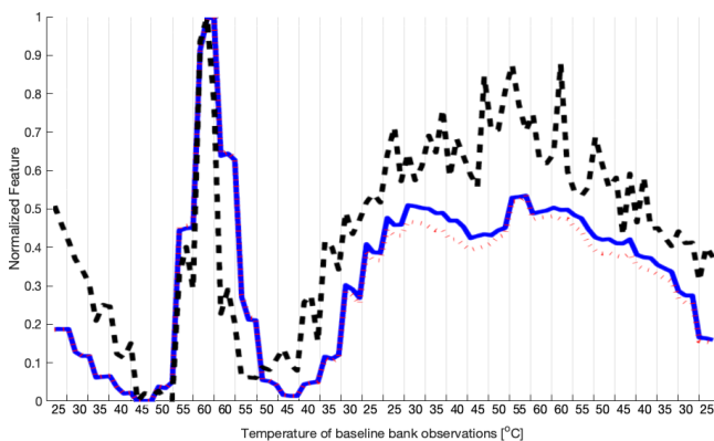
Figure 25. Differential features comparison: D2 at 35°C in case study 1.
