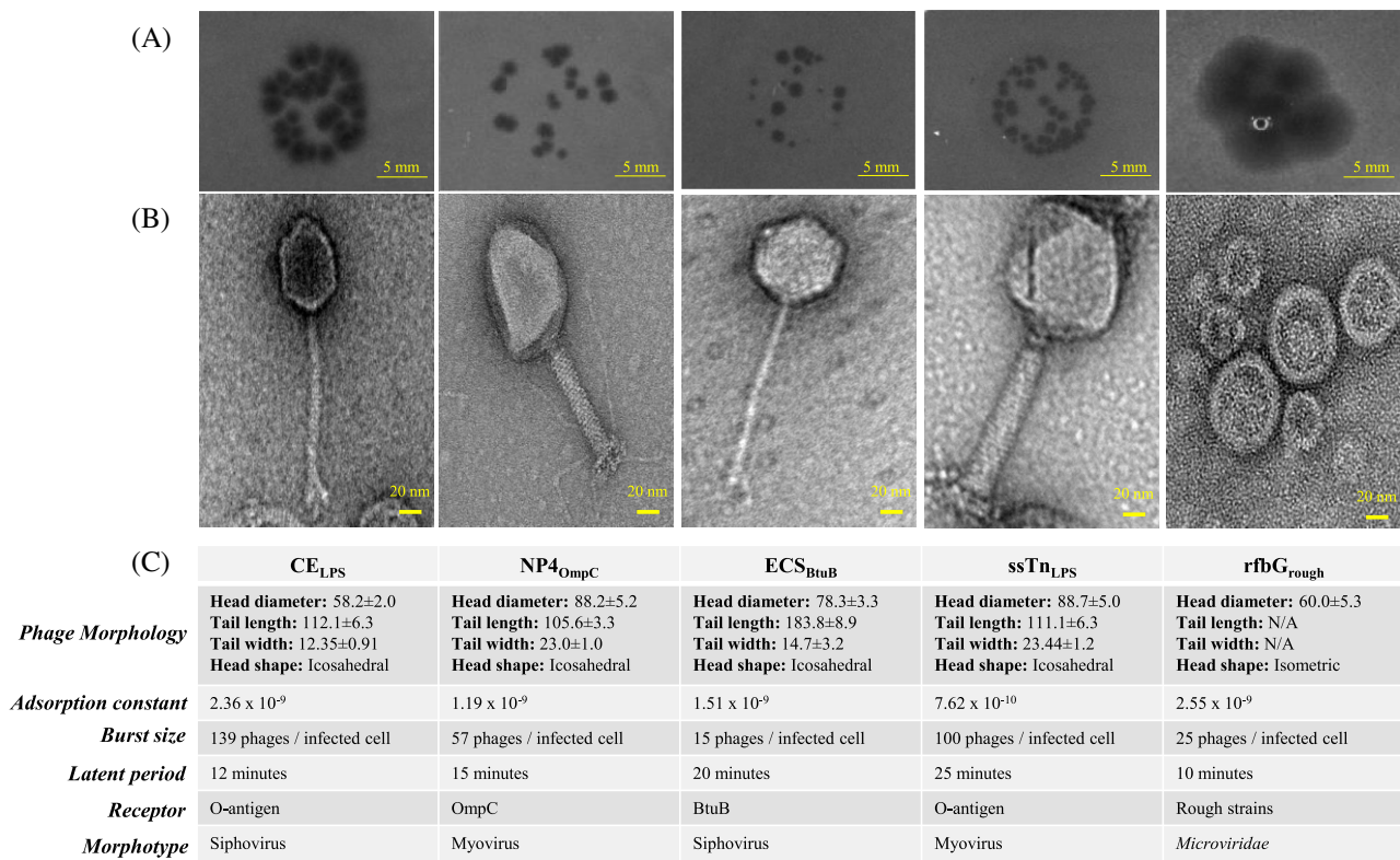
Figure 4. Salmonella phages selected for cocktail composition. (A) Plaques on the respective propagation hosts (Table S5). (B) Transmission electron micrographs. (C) Table of phage features.
