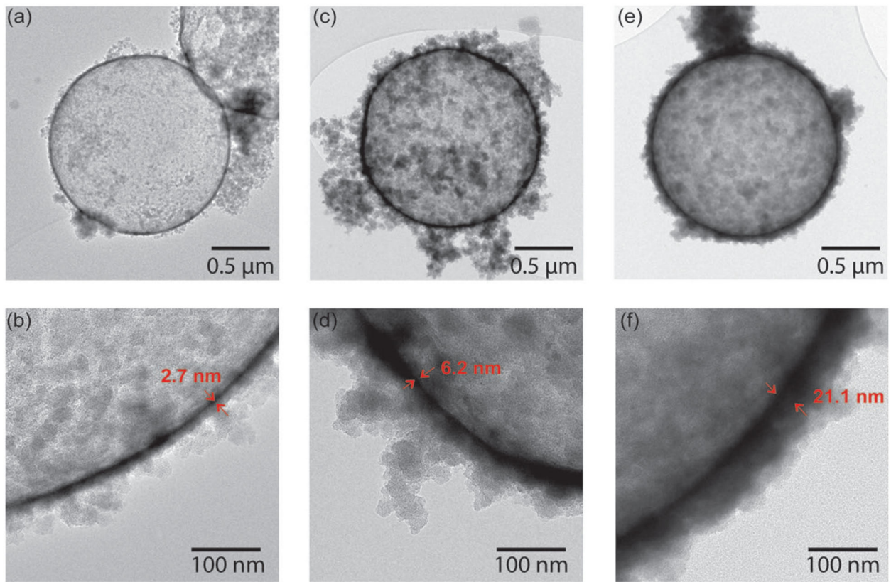
Figure 1. TEM images of iron (III) doped silica hollow shells. a,b) ultrathin, c,d) medium-thickness, and e,f) thick iron (III) doped silica shells.
