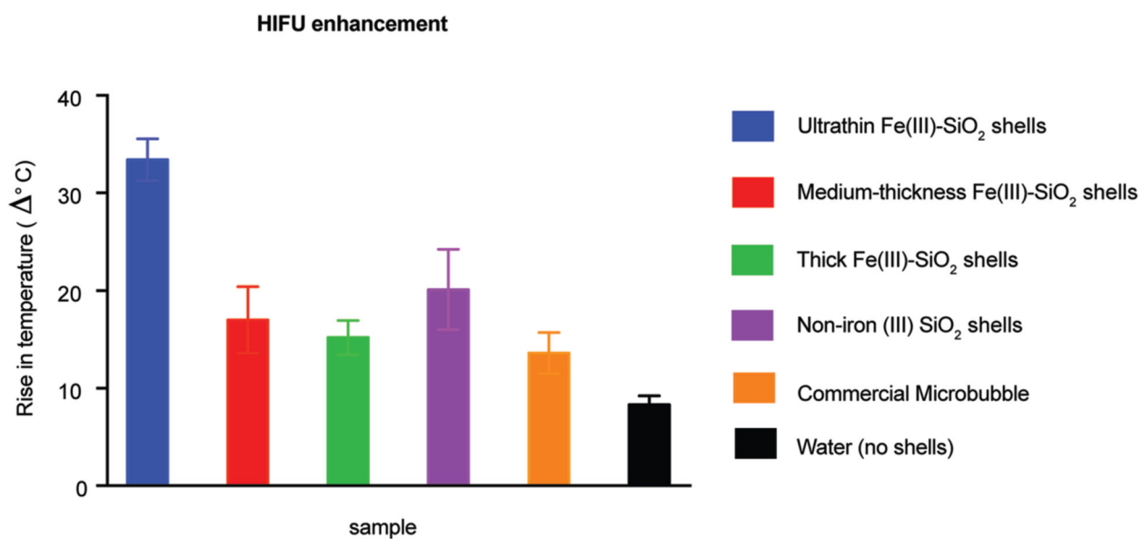
Figure 4. HIFU response of iron (III) doped silica shells, non-iron (III) doped silica shells, commercial microbubbles, and absence of shells (pure water). 0.4 \text{ mg mL}^{-1} silica shells or Definity microbubbles at the same gas volume were applied HIFU (100 Watts) at 100% duty cycle for 10 s.
