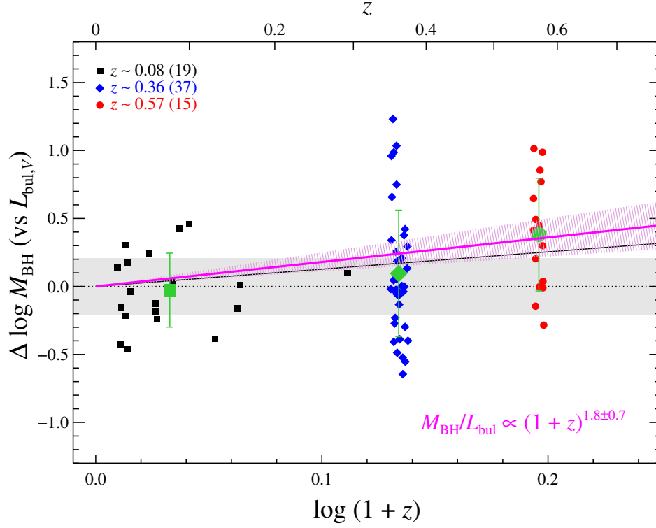
Figure 5. Redshift evolution of the offset in \log M_{\text{BH}} for a given L_{\text{bul}} with respect to local baseline M_{\text{BH}} - L_{\text{bul}} relation (black dotted line with gray shaded region showing the intrinsic scatter). Colored symbols indicate local RM AGNs (black squares at \bar{z} \sim 0.08 ) and our intermediate- z sample at z = 0.36 (blue diamonds) and at z = 0.57 (red circles). The mean and root-mean-square (rms) scatter of offsets for each sample are shown as green big symbols with error bars. The black solid line represents the best-fit trend for all intermediate- z objects in the functional form of \Delta \log M_{\text{BH}} = \gamma \log(1+z) without taking into account for selection effects. The magenta solid line with the hatched 1\sigma confidence range shows the result when taking into account selection effects. The corresponding best-fit value for the evolution slope is given in the lower right corner.
