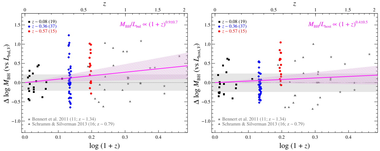
Figure 8. Same as Figure 5, but with the additional samples from Bennert et al. (2011b) and Schramm & Silverman (2013). Left (right) panel shows the evolution of the mass offset for a given L_{\text{bul}} ( L_{\text{host}} ) with respect to the local baseline M_{\text{BH}} - L_{\text{bul}} ( M_{\text{BH}} - L_{\text{host}} ) relation. The best-fit evolution slope ( \gamma ) estimated from the Monte Carlo simulation incorporating selection effects is given at each upper right corner and over-plotted as a magenta solid line with a hatched 1\sigma confidence range.
