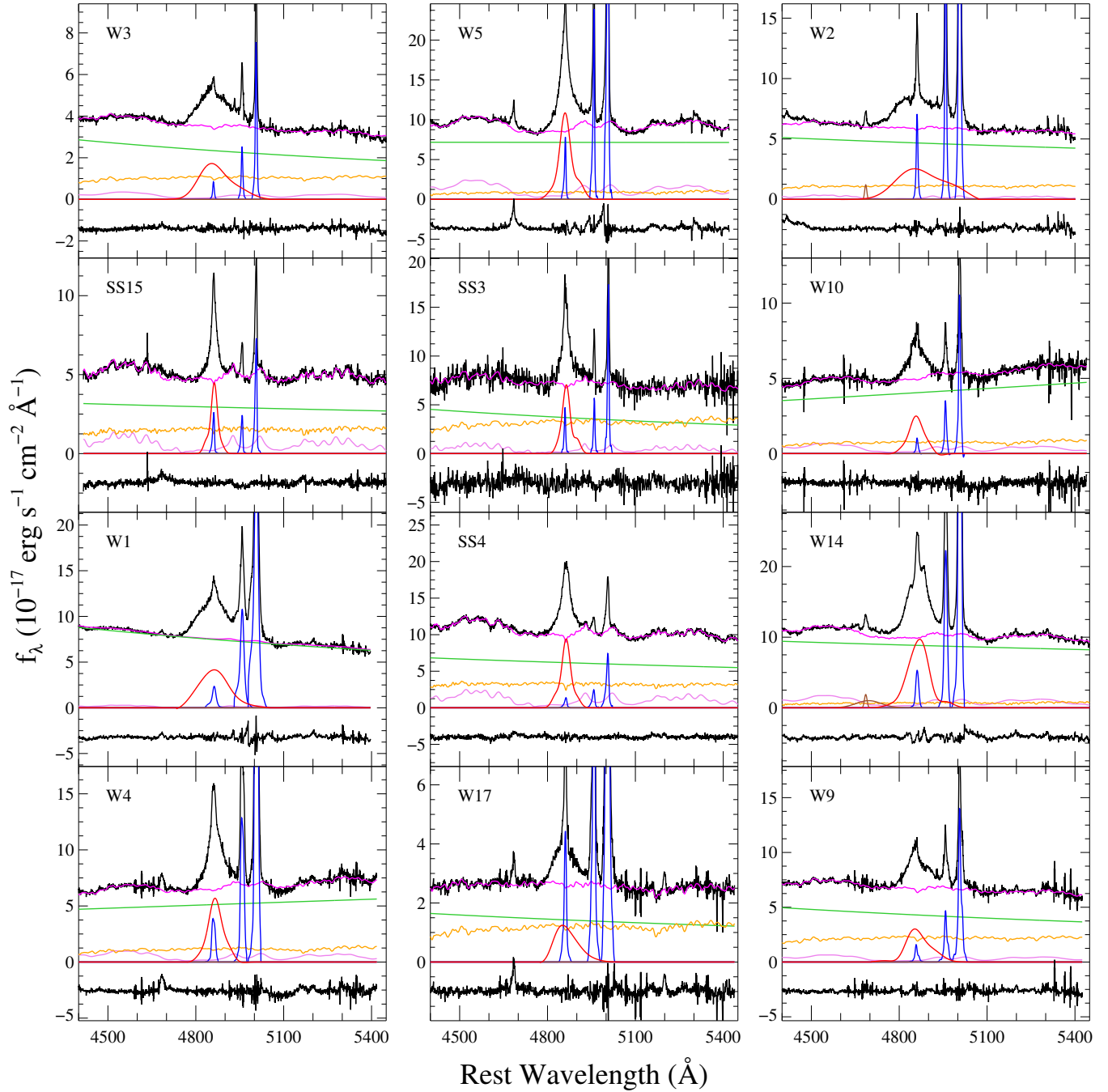
Figure 1. Multi-component spectral decomposition for 12 objects. The observed spectra are shown along with the best-fit models. In each panel, observed spectra (black) and the continuum+Fe II+stellar best-fit model (magenta) are shown in the upper part, and the best-fit power-law continuum (green), stellar template (yellow), and Fe II template (violet) models are presented in the middle part. Three narrow lines [ \text{H}\beta , [\text{O III}] \lambda\lambda 4959, 5007 (blue)], broad \text{H}\beta (red), and the broad and narrow \text{He II } \lambda 4686 components (brown; only included if blended with \text{H}\beta ) are presented in the bottom part. The residuals (black), representing the difference between the observed spectra and the sum of all model components, are arbitrarily shifted downward for clarity.
