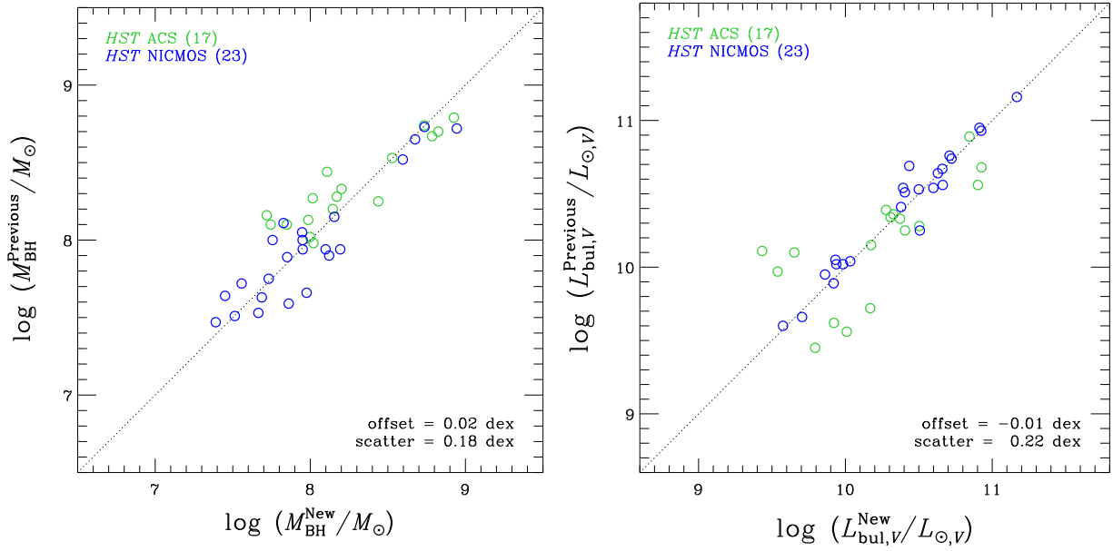
Figure A3. Difference of BH mass estimates (left) and bulge luminosity estimates (right) between previous results (Bennert et al. 2010) and new results presented here.
