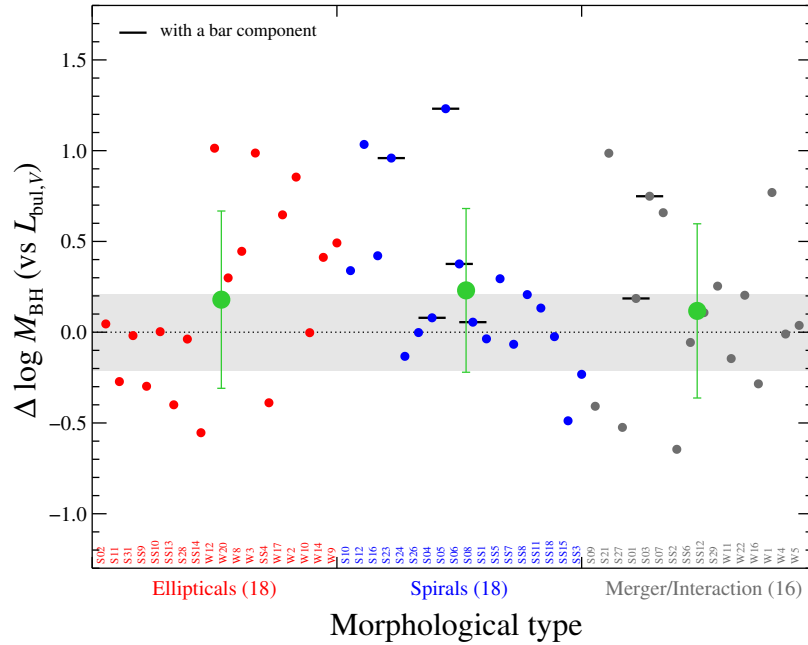
Figure 6. The measured offset in \log M_{\text{BH}} for a given L_{\text{bul}} with respect to local baseline M_{\text{BH}} - L_{\text{bul}} relation (black dotted line with gray shaded region for the intrinsic scatter) with simple morphological type classification based on the visual inspection of HST images. Objects containing a bar component are indicated with a black horizontal bar.
