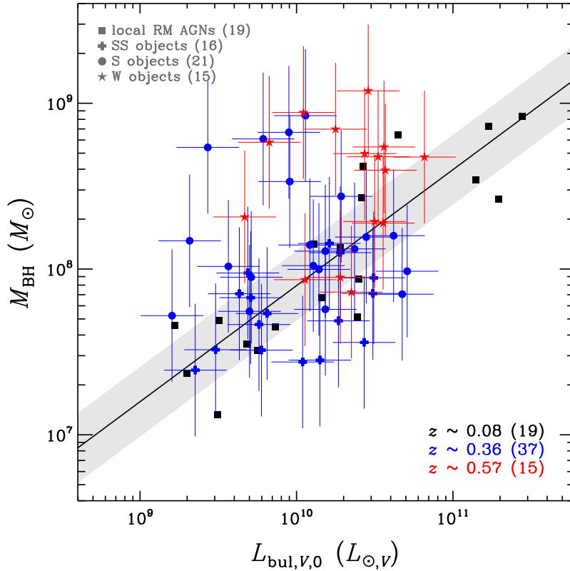
Figure 4. M_{\text{BH}}-L_{\text{bul}} relation. Colored symbols indicate our intermediate- z sample (plus signs: SS objects; circles: S objects; stars: W objects; see Sec. 2.1 for the details of the sample). Corresponding redshifts of the samples are expressed by different colors (black: local ( \bar{z} \sim 0.08 ); blue: z = 0.36 ; red: z = 0.57 ). The black filled squares are the local RM AGNs taken from Bennert et al. (2010) with the best-fit relation (black solid line) and its intrinsic scatter (0.21 dex; gray shaded region).
