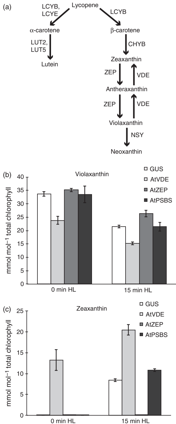
Figure 2. Xanthophyll accumulation in N. benthamiana leaf spots over-expressing Arabidopsis thaliana NPO-related genes. (a) Schematic diagram of a portion of the carotenoid biosynthetic pathway. Lycopene \beta -cyclase, LYCB; lycopene \epsilon -cyclase, LYCE; \beta -carotene hydroxylase, CHYB; \epsilon -ring hydroxylase, LUT2; violaxanthin de-epoxidase, VDE; zeaxanthin epoxidase, ZEP; neoxanthin synthase, NSY. (b, c) (b) Violaxanthin and (c) zeaxanthin accumulation in leaf spots over-expressing AtPSBS , AtVDE , or AtZEP with GUS as a negative control at time zero and after 15 min of high light treatment ( 600 \mu\text{mol photons m}^{-2} \text{sec}^{-1} ). Error bars represent standard deviation ( n = 4 ).
