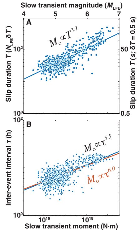
Fig. 4. Moment scaling of slow transients in Guerrero as inferred from LFEs.
