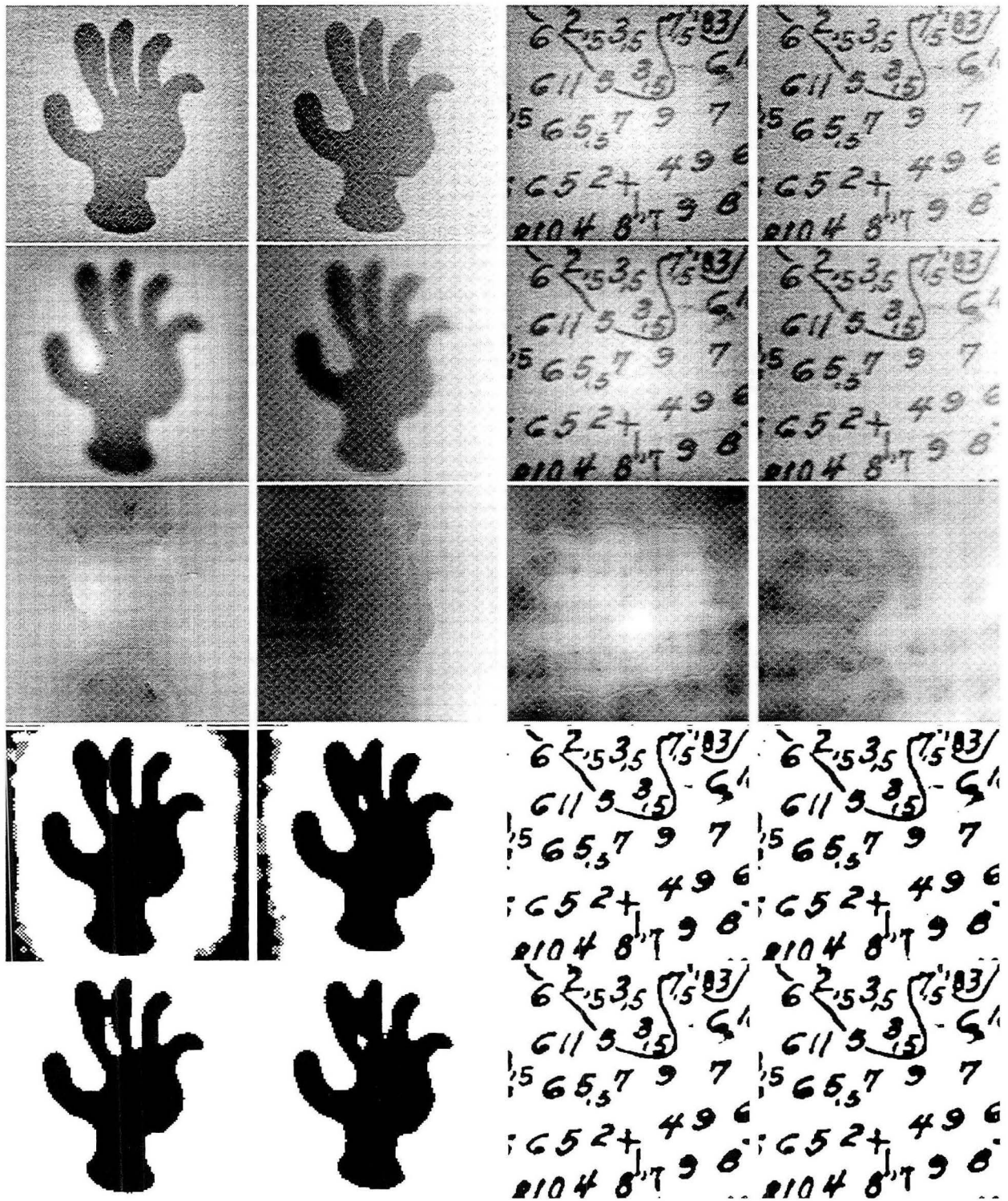
Figure 7: Rows top to bottom: 1. Original image + noise + smooth function. An intensity plane I + x is added to the right, and I + \sin(x) \sin(y) to the left of each pair. 2. Smoothed image. 3. Threshold surface. 4. Binarization before validation. 5. Binarization after validation.
