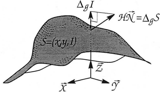
Figure 3: Consider the mean curvature H in the surface normal direction \vec{N} . It can also be expressed as H\vec{N} = \Delta_g \mathcal{S} . Beltrami operator that operates on I : \Delta_g I , is the third component of this vector: Projection onto the I ( \vec{Z} ) direction.
