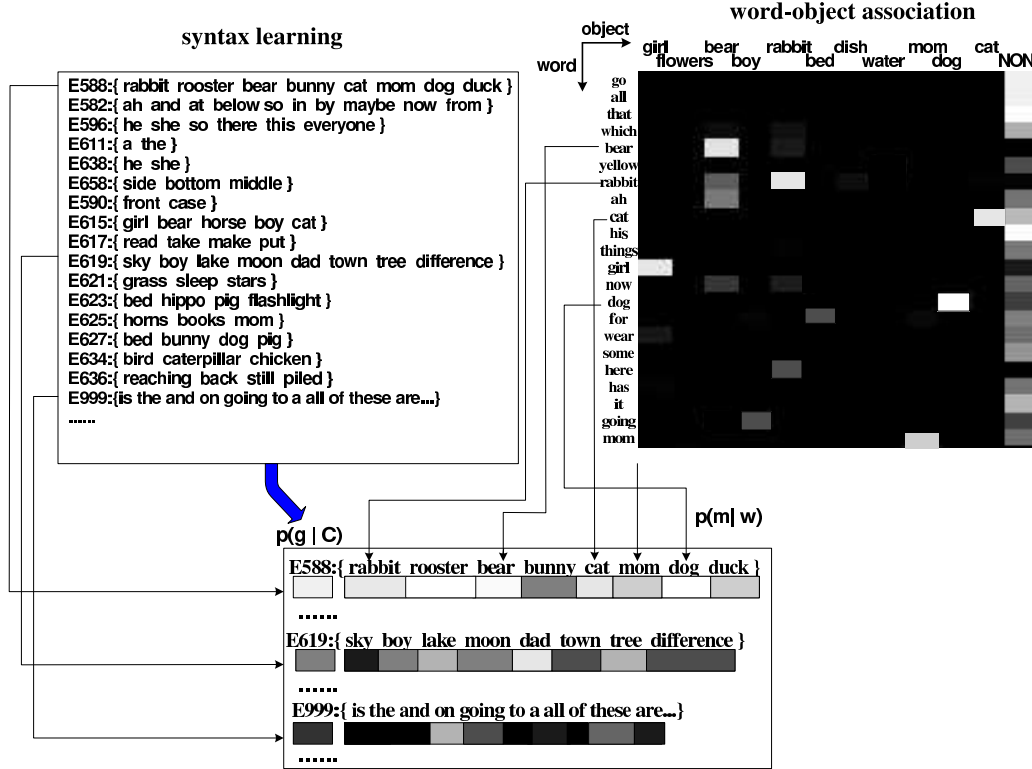
Figure 1: Learning syntax-semantic mappings. Upper left: the syntax learning process categorizes words into several syntactic groups. Upper right: the word-learning process estimates the association probabilities of any co-occurring word-object pairs represented by cells in the figure. White color means high association probabilities and dark color means low association probabilities. Bottom: the integration of semantic and syntactic knowledge results in p(g|C) – the semantic property of each syntactic class. p(g|C) can then be used to improve the estimates of word-object association probabilities by considering semantic properties of other words in the same groups.
