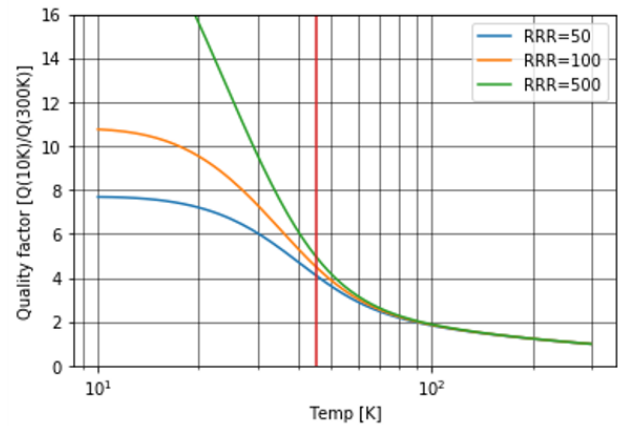
Figure 2: Quality factor predictions for an analytic cavity based on NIST material data. The red vertical line indicates the 45 K operating point intended for our first cryostat.
