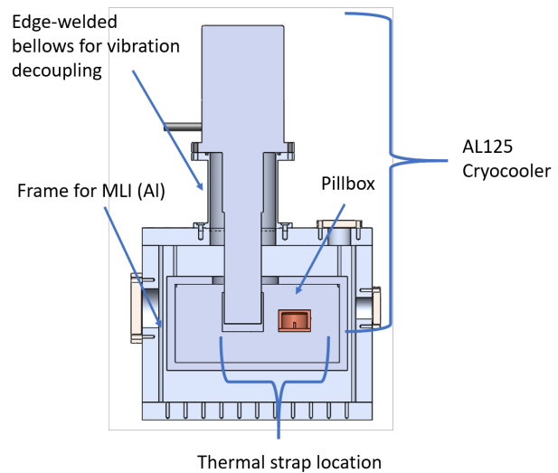
Figure 5: Simple cube shaped vacuum cryostat for initial tests including lower power RF and cathode thermal stress measurements.
