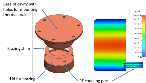
Figure 3: Brazed pillbox assembly.
