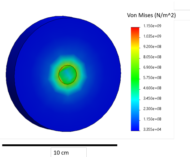
Figure 4: Stress calculations for annulus of copper with molybdenum cylinder within when cooled from 300 to 45 K. The outer annulus is 10 cm in diameter and the inner Mo cylinder is 1.676 cm in diameter in order to approximate the 1/2 cell backplane and cathode plug.
