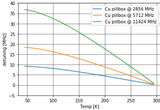
Figure 1: Cavity detuning due to temperature changes at different frequencies of operation.
