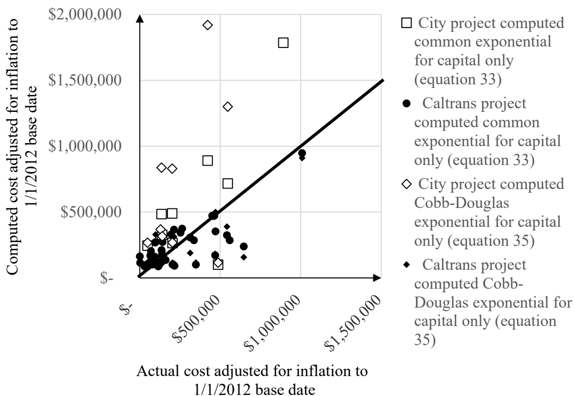
Figure 4-2 Actual versus computed project costs for construction capital only adjusted for inflation to 1/1/2012 base date
