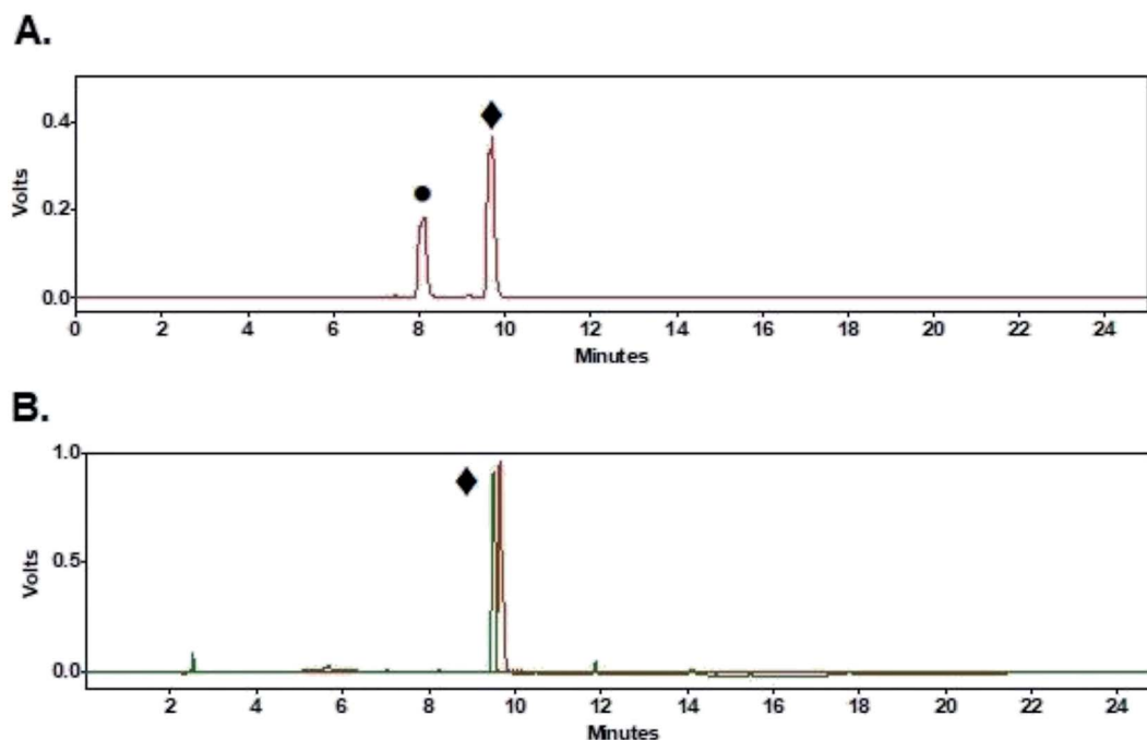
Fig. 6 HPLC chromatogram of radiolabeled [^{18}\text{F}]\text{FPy-YGGFL} (6) (PMT(gamma)-red, UV(220 nm)-green). (A) Crude radioHPLC chromatogram (peak ●-6- [^{18}\text{F}]\text{fluoronicotinic acid} , peak ◆- [^{18}\text{F}]\text{FPy-YGGFL} (6)). (B) Purified HPLC chromatogram co-injected with [^{19}\text{F}]\text{FPy-YGGFL} (peak ●- [^{19}\text{F}]\text{FPy-YGGFL} (6)).
