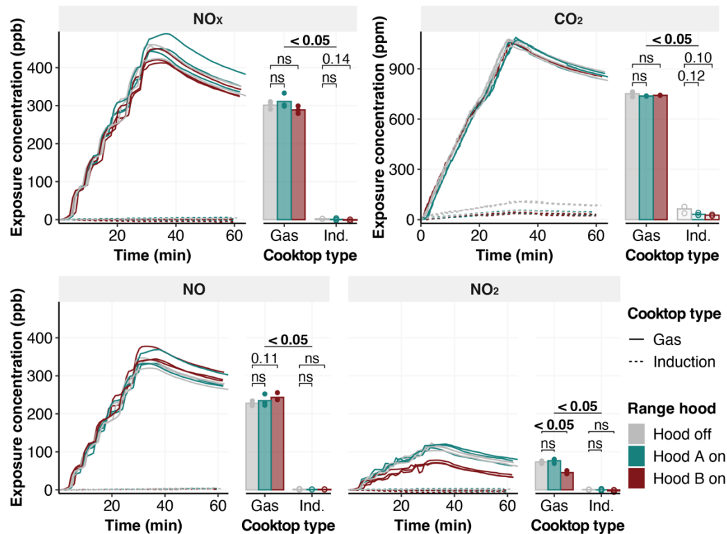
Figure 5. Time-resolved and averaged exposure concentrations of \text{NO}_x , \text{NO} , \text{NO}_2 , and \text{CO}_2 during gas and induction cooking under three range hood conditions. Each solid or hollow point represents the average net exposure concentration during the exposure period of each experiment.
