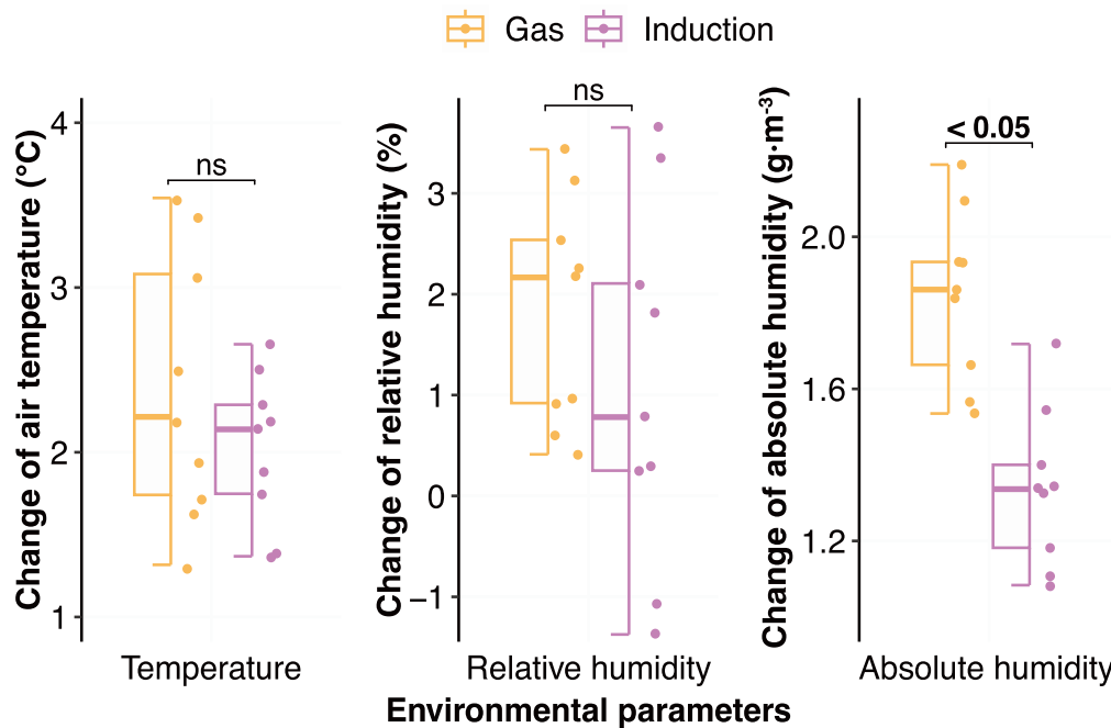
Figure 3. Average changes in temperature, relative humidity, and absolute humidity relative to the reference period for each test. Comparisons show p -values calculated with Welch's t -test; “ns” indicates a non-significant difference, with p -value > 0.15 .
