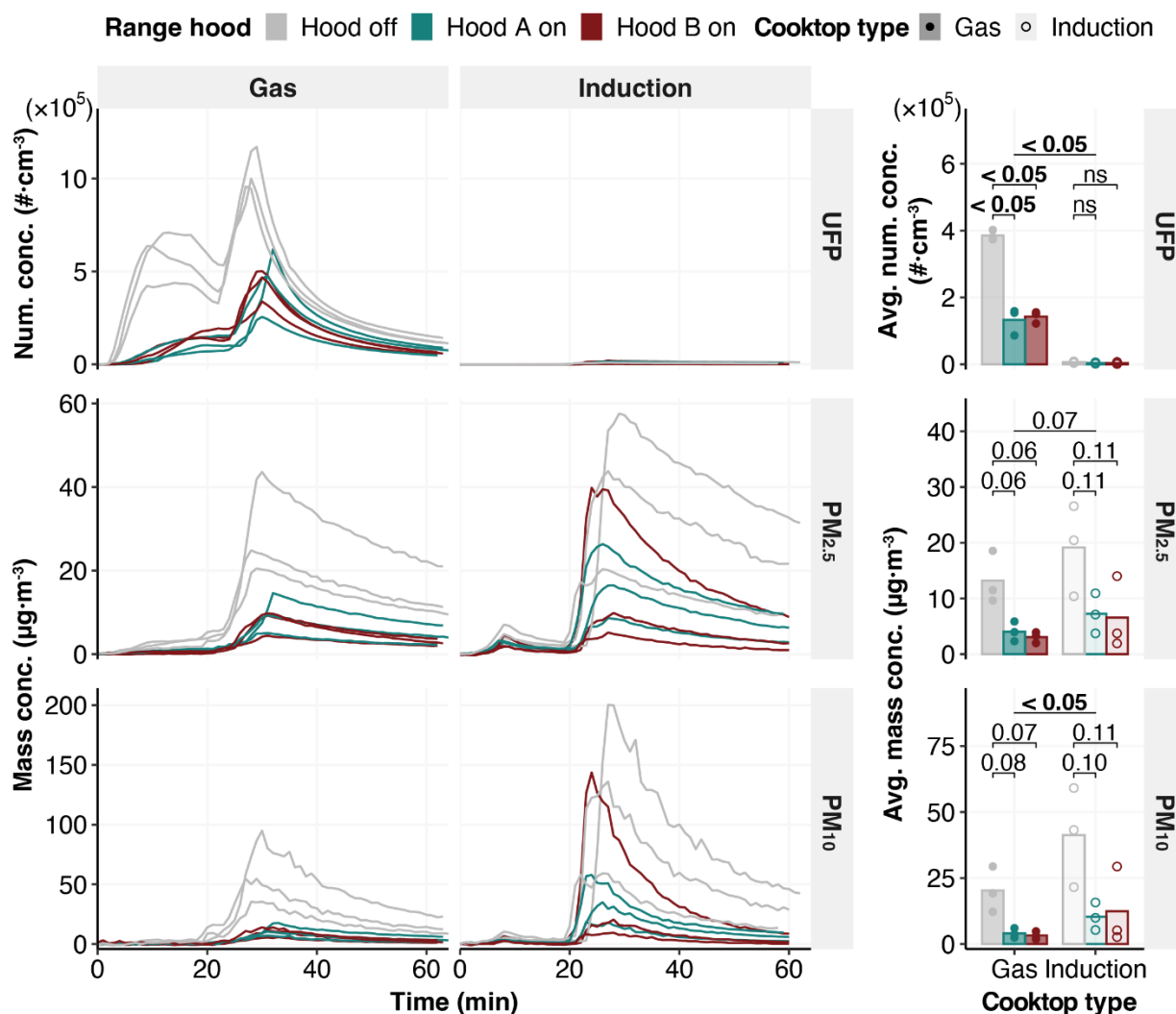
Figure 6. Time-resolved (left) and time-averaged (columns at right) exposure concentrations of UFPs, \text{PM}_{2.5} , and \text{PM}_{10} during gas and induction cooking under three range hood conditions.
