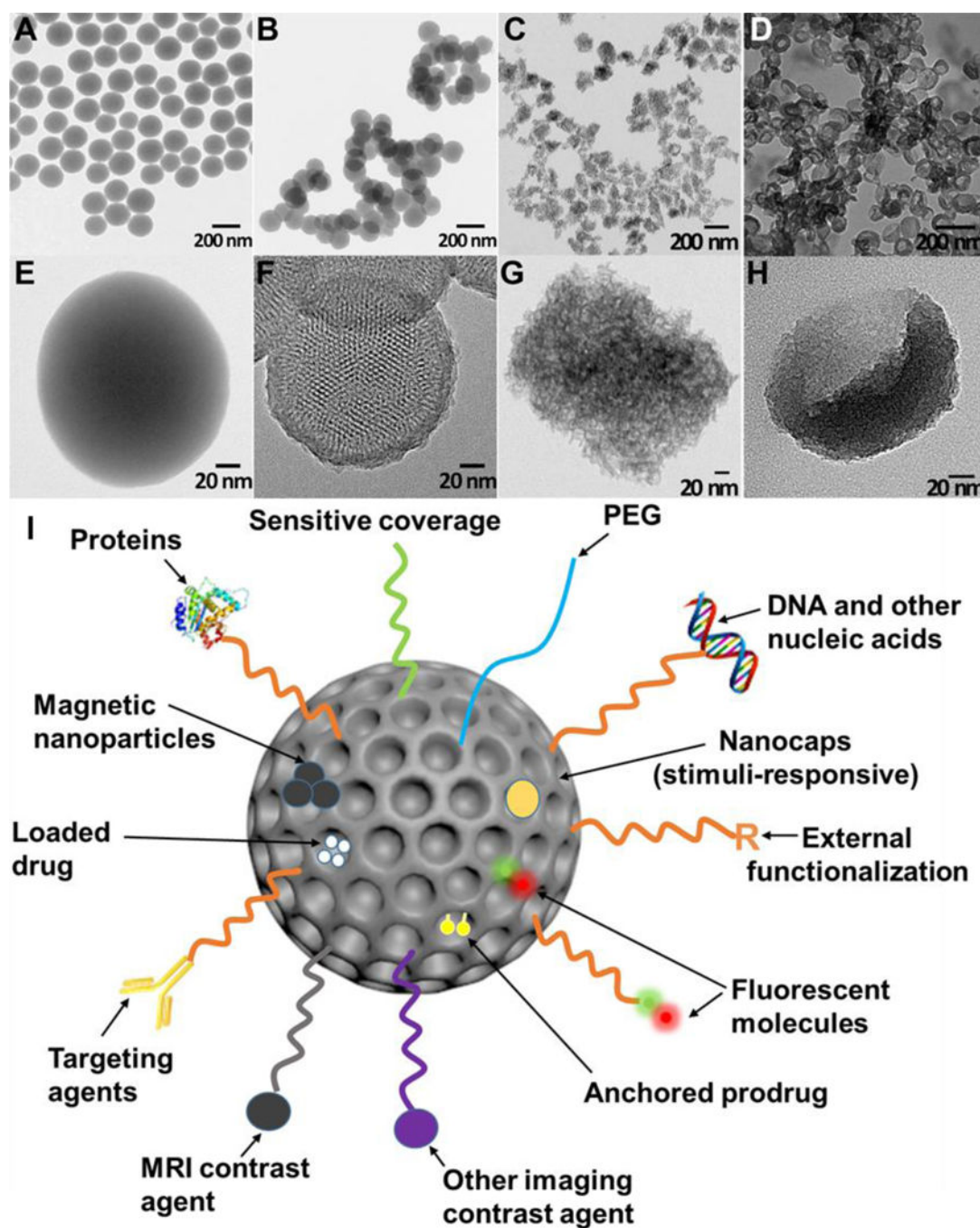
Figure 3. TEM images of solid Stöber silica nanoparticles (A, E), MCM-41 mesoporous silica nanoparticles (B, F), mesocellular foam silica nanoparticles (C, G), and exosome-like silica nanoparticles (D, H) (Adapted from reference 31 ). (I) Multifunctionality of silica nanoparticles. PEG is polyethylene glycol.
