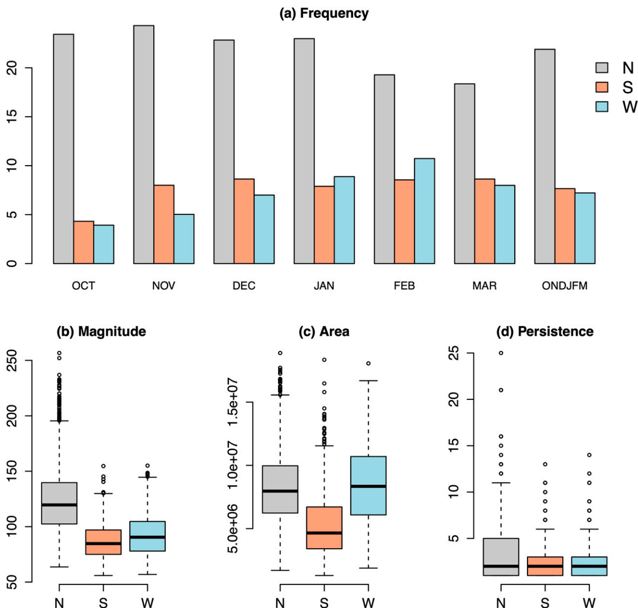
FIG. 4. Distributions of ridge characteristics for N-, S-, and W-ridge types: (a) frequency (percentage occurrence from all time steps), (b) magnitude (m), (c) area ( \text{km}^2 ), and (d) persistence (days). These characteristics were generated from 20CRV2c over the period 1950–2014 for months October–March. Boxplot components are horizontal line (median), boxes [interquartile range (IQR)], whiskers (1.5IQR), and outliers/circles ( > 1.5\text{IQR} ).
