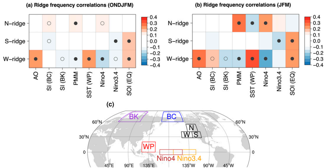
FIG. 8. Pearson correlation coefficients between monthly ridge frequency anomalies and various remote drivers/modes of variability (x axis): the Arctic Oscillation (AO), sea ice variability over the Bering–Chukchi (BC) and the Barents–Kara (BK) regions, the Pacific meridional mode (PMM), SSTs in the western Pacific (SST WP), the Niño-4 index, the Niño-3.4 index, and the equatorial Southern Oscillation index (SOI-EQ.). Correlations are shown for (a) October–March and (b) January–March; p values < 0.05 are indicated by open circles and p values < 0.01 are indicated by filled circles. The time period is 1950–2014 with ridge types generated from 20CRV2c. (c) The locations of select regions to aid interpretation. Figures S11 and S12 also show these associations, but for ridge persistence and ridge magnitude, respectively.
