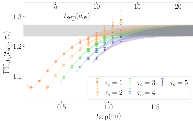
FIG. 2. We plot the numerical FH_{A_3}(t_{sep}, \tau_c) data for various values of \tau_c as well as the posterior reconstruction of these correlation functions from the global analysis that uses \tau_c = 1 .
