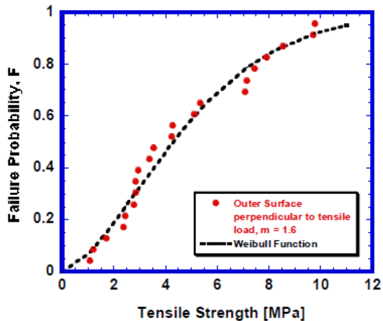
Figure 2.22: Weibull distribution of tensile strength perpendicular to layered structure (source: Lin [65]).
