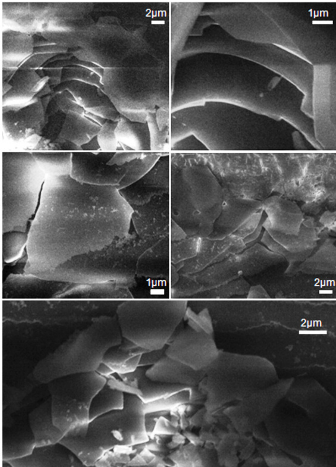
Figure 4.40: SEM micrographs of deproteinized nacre tested at the top surface. Debris and brittle fracture can be observed on deproteinized nacre.
