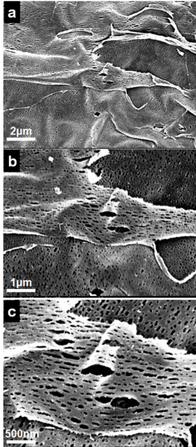
Figure 4.27: a) Top view of the interlayers stacked upon one another. This section of the demineralized nacre was taken near the gauge cross-section where most of the damage due to the mechanical testing was done. b) Close-up view showing the tear of the layer and c) Elongated and torn holes in the nanolayer.
