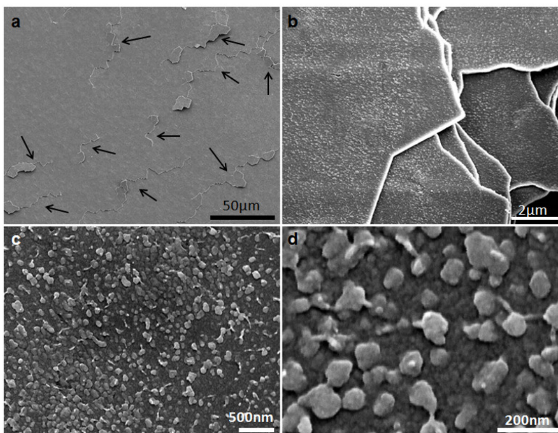
Figure 4.34: ‘Birds-eye-view’ of fracture surface showing different tile layers peeled off as load is applied. Nanoasperities that cover the surface with a uniform distribution
