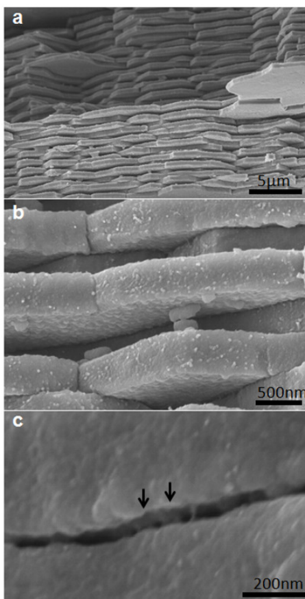
Figure 4.33: a) Cross-sectional view of the nacre post-deproteinization retaining the structure of the mineral tiles (~400-500nm in thickness). b) and c) Neighboring tiles exposing nanoasperities on upper and lower tablet.
