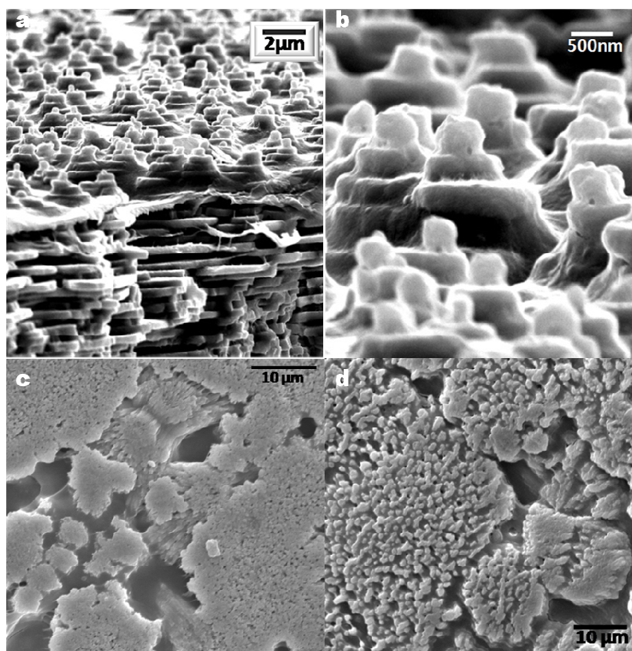
Figure 4.4: Sequential growth results after 3 weeks of implantation. a) Growth at 21 °C with abalone regularly fed (cross-section); b) Detailed view of aragonite tile morphology; c) Growth in 15 °C with abalone regularly fed; d) Growth in 20 °C without food available.
