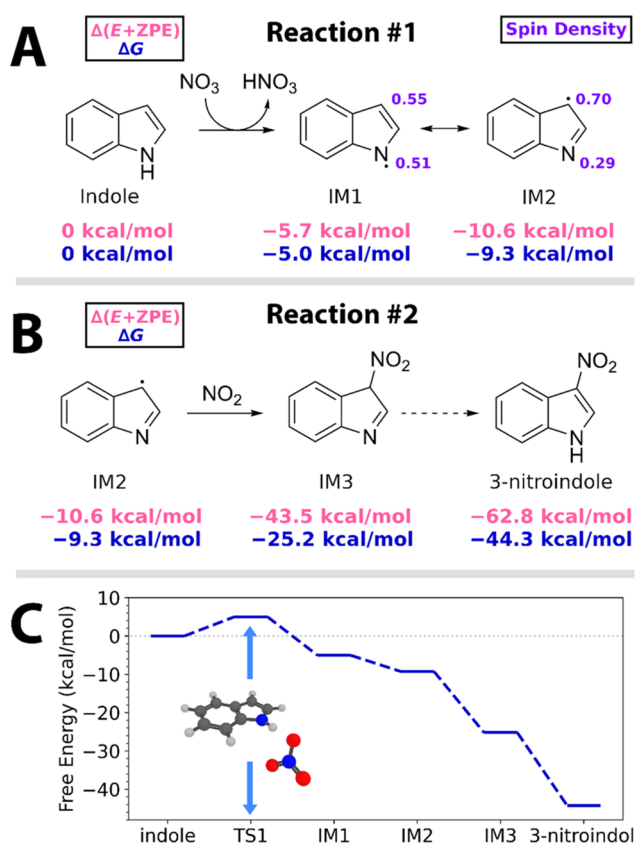
Figure 5. Thermochemical results at the PBE0/6-311++G(d,p) level for the hydrogen abstraction mechanism initiated by removal of the hydrogen at the N position (N1). \Delta(E + ZPE) values are provided in pink, and \Delta G values are provided in blue, with reference to the reactants (including the oxidant) in each reaction.
