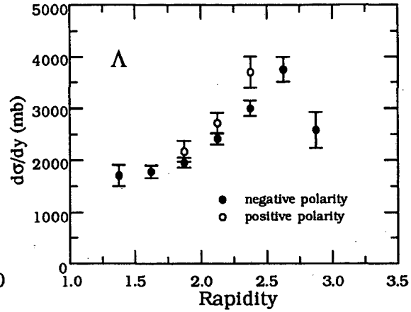
Fig. 18 Positive and negative polarity data.
