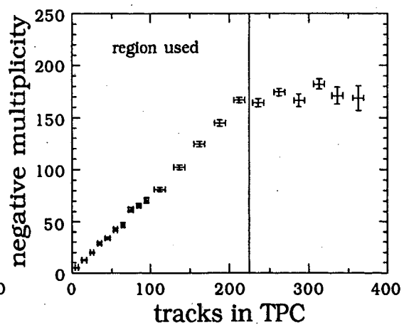
Fig.11. Determination of negative multiplicity.
