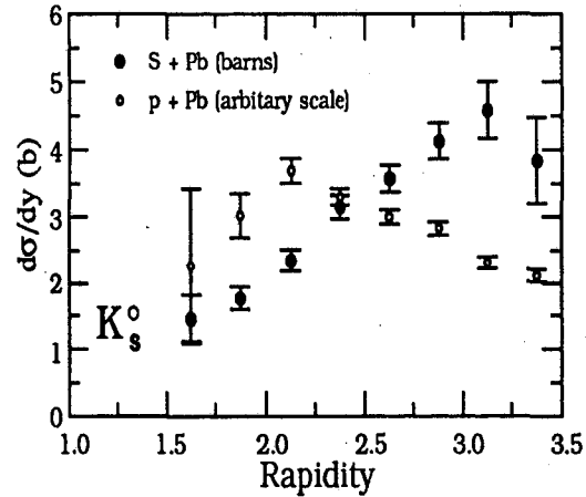
Fig. 19b K^0 rapidity distributions.
