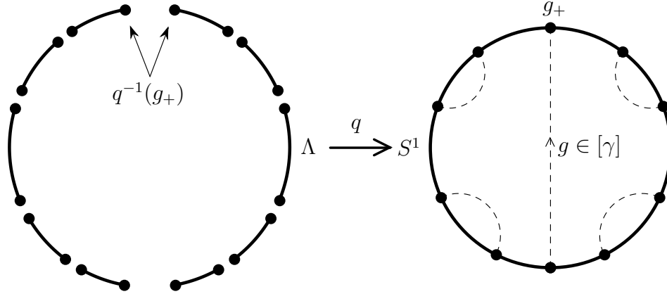
Figure 4: Denjoy blow-up.
