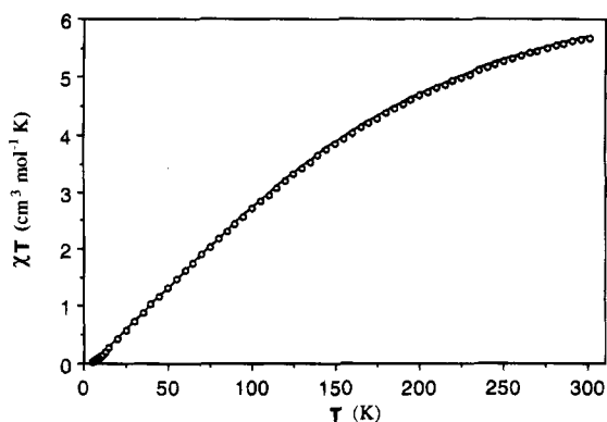
Figure 1. Experimental (○) plot of \chi_m T versus T for a polycrystalline sample of [\text{Fe}^{\text{III}}\text{Mn}^{\text{II}}\text{BPMP}(\text{O}_2\text{CCH}_3)_2](\text{BPh}_4)_2 with the theoretical curve (—) generated from the Hamiltonian H = JS_{\text{Fe}} \cdot S_{\text{Mn}} + \beta(S_{\text{Fe}} \cdot g_{\text{Fe}} + S_{\text{Mn}} \cdot g_{\text{Mn}}) \cdot B using J = 23 \text{ cm}^{-1} , g_{\text{av}} = 2.0 for Fe(III) and Mn(II).
