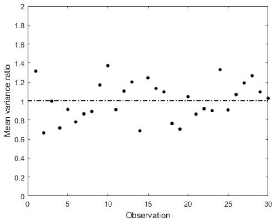
Figure 8. Ratio of the average curvature variance in outputs from the computational model to outputs in the detector model. Each point is the ratio for one of the 30 shapes in our test, and the dashed line show the mean ratio across all 30 shapes.
