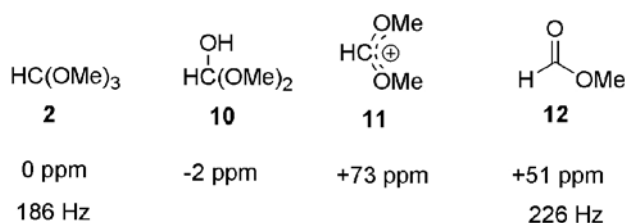
Figure 8. Calculated chemical shifts relative to 2 and experimental 1 J CH couplings for possible resting-state species for the catalysis in 1 .
