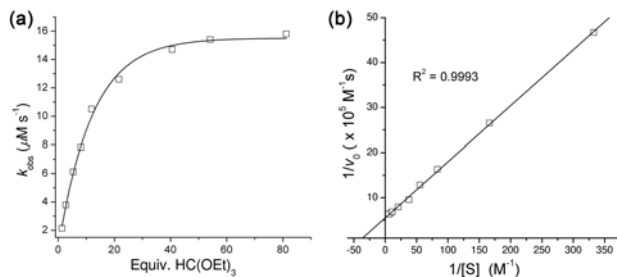
Figure 4. Rate dependence on [3] with catalytic 1 in \text{H}_2\text{O} pH = 11.0, 100 mM \text{K}_2\text{CO}_3 , 50 °C. Substrate saturation (a) is observed. The corresponding Lineweaver-Burke plot (b). Modified from reference 50.
