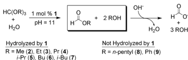
Figure 2. Scope of orthoformates investigated in 1 .
