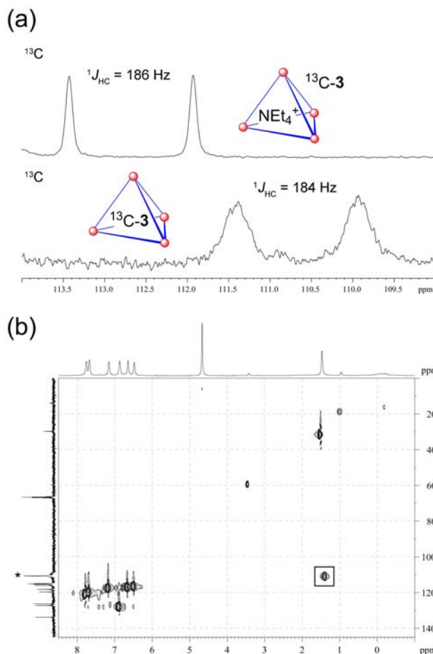
Figure 9. (a) ^{13}\text{C} NMR spectrum of ^{13}\text{C} -3 with (\text{NEt}_4)_{11}[\text{NEt}_4 \subset \mathbf{1}] in \text{D}_2\text{O} (top), and ^{13}\text{C} NMR spectrum of [\text{C}^{13}\text{-3} \subset \mathbf{1}]^{12-} in \text{D}_2\text{O} (bottom). (b) ^1\text{H} - ^{13}\text{C}\{^1\text{H}\} HSQC NMR spectrum showing correlation between the C-H (*) of encapsulated ^{13}\text{C} -3.
