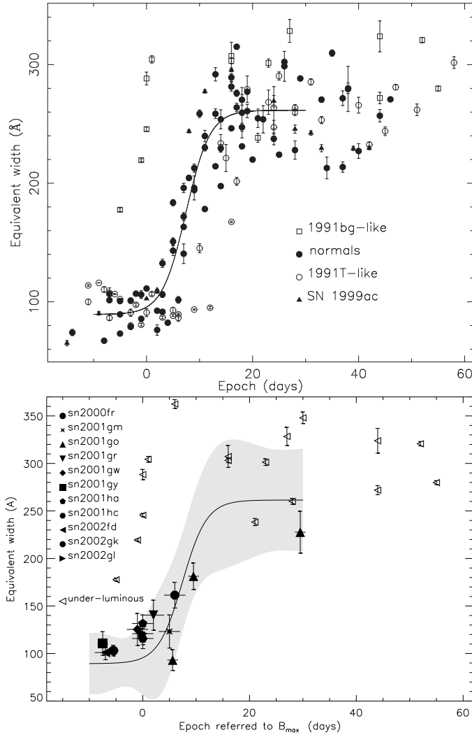
Fig. 6 “Mg II 4300” Upper Panel: Measured pseudo-equivalent widths corresponding to “Mg II 4300” (#3). SN 1991bg-like objects are marked with open squares, 1991T-like SNe Ia with open circles, normal SNe Ia with filled circles and SN 1999ac with triangles. Error-bars include the error described by Eqn. 2 as well as systematic uncertainties arising from the pseudo-continuum fit. The solid line represents the average behavior of normal SNe Ia, as described in Eqn. 3 with \theta=(172.2, 89.4, 7.5, 2.5) . In general, 1991bg-like SNe Ia lie above the average curve whereas 1991T-like SNe Ia lie below it. Lower Panel: A comparison between the ‘Mg II 4300’ pseudo-EWs in low- and high-redshift SNe Ia. High-redshift supernova are indicated by large filled symbols. The gray filled area represents the 95% probability region for normal low-redshift SNe Ia. Peculiar under-luminous nearby SNe Ia are shown separately for comparison. See text for details.
