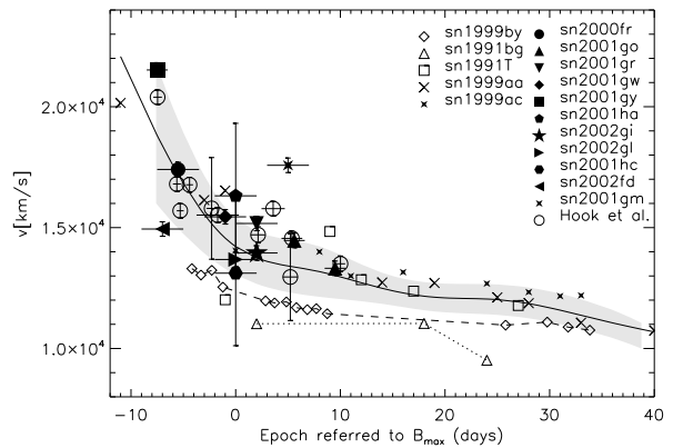
Fig. 4 The change in the blueshifts of the Ca II H&K absorption minimum with epoch for a sample of high-redshift SNe Ia (presented in section 3, filled symbols, and from Hook et al. (2005) open circles) and a sample of low-redshift SNe Ia. The dashed and dotted lines indicate the values of extremely under-luminous SNe Ia SN 1999by (Garnavich et al. 2004) and SN 1991bg (Leibundgut et al. 1993) respectively. The solid line indicates the average trend for Ca II H&K, which has been computed using a large data set of low-redshift normal SNe Ia (Garavini et al. 2004). The gray band shows the dispersion (1 standard deviation) of the data about the average trend.
