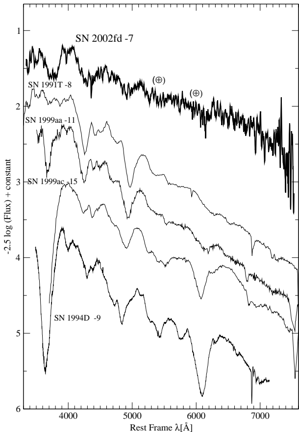
Fig. 3 SN 2002fd at day -7 , re-binned to 20 \text{ \AA} per pixel (thick solid line), compared to normal and peculiar SNe Ia. The \oplus symbols mark regions of strong telluric absorption.
