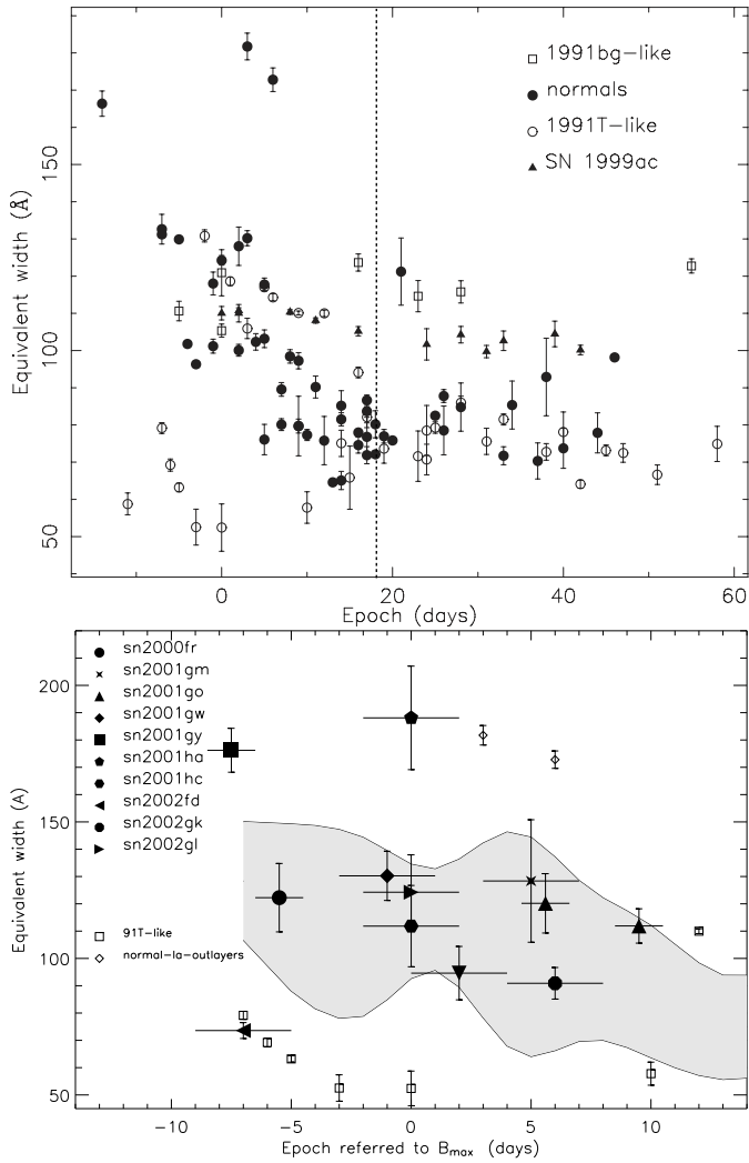
Fig. 8 “Ca II H&K” Upper Panel: Measured pseudo-equivalent widths corresponding to “Ca II H&K” (#1). SN 1991bg-like objects are marked with open squares, 1991T-like SNe Ia with open circles, normal SNe Ia with filled circles and SN 1999ac with triangles. Error-bars include the error described by Eqn. 2 as well as systematic uncertainties arising from the pseudo-continuum fit. The vertical dashed line indicates the upper epoch limit in the lower panel. Lower Panel: A comparison between the ‘Ca II H&K’ pseudo-EWs in low- and high-redshift SNe Ia. High-redshift supernova are indicated by large filled symbols. The gray filled area represents the 95% probability region for normal (non-outliers) and the under-luminous low-redshift SNe Ia SN 1999by, SN 1991bg and SN 1986G. Outliers normal SNe Ia are indicated with the diamond symbols. Slow declining SNe Ia are indicated by the open square symbols.
