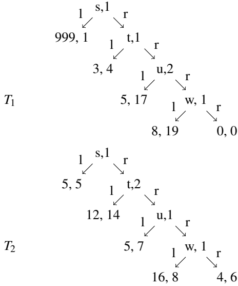
Figure 3: Two \Lambda_3^1 trees.
