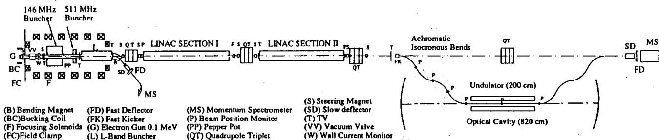
Fig. 1 Layout of the accelerator - FEL system.
