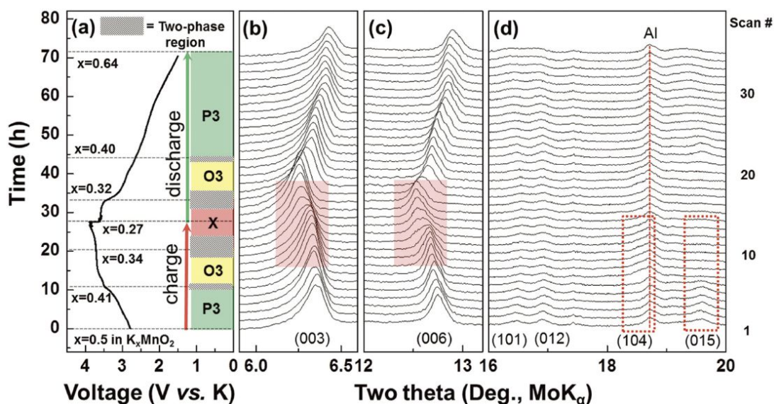
Fig. 19 Structural changes of P3-K 0.5 MnO 2 during charge and discharge. (a) Typical charge/discharge profiles of P3-type K 0.5 MnO 2 at a current rate of 2 mA g -1 . (b–d) In situ XRD pattern taken for 2 h scanning rate per pattern. Reproduced from Refs. 31 With permission of Wiley.
