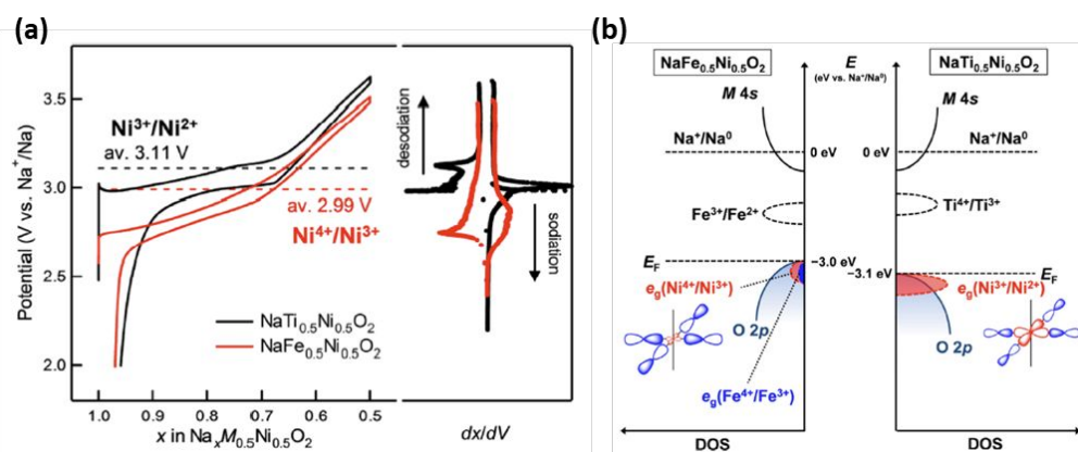
Fig. 4 (a) Potential profiles as a function of x in \text{Na}_x\text{Ti}_{0.5}\text{Ni}_{0.5}\text{O}_2 and \text{Na}_x\text{Fe}_{0.5}\text{Ni}_{0.5}\text{O}_2 . The dx/dV plots are also shown for comparison. (b) Schematic electronic structures of \text{Na}_x\text{M}_{0.5}\text{Ni}_{0.5}\text{O}_2 ( M = \text{Ti}, \text{Fe} ). Oxygen 2p and Ni e_g orbitals hybridize well to delocalize holes over both Ni and oxygen in \text{Na}_x\text{Ti}_{0.5}\text{Ni}_{0.5}\text{O}_2 . For \text{Na}_x\text{Fe}_{0.5}\text{Ni}_{0.5}\text{O}_2 , the frontier orbital with a dominant oxygen 2p character does not reflect the \text{Ni}^{4+}/\text{Ni}^{3+} character significantly. Reproduced from Refs. 63 With permission of ACS.
