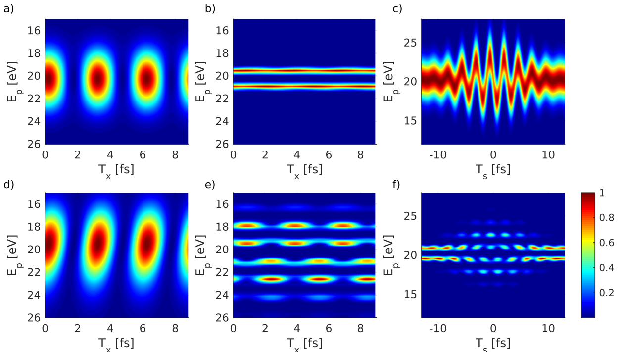
FIG. 2. Comparison of TRPES in a purely electronic (atomic) system for different pulse parameters: (a) \sigma_x=0.5 fs, the beating caused by the coherence is well resolved in the time domain. (b) \sigma_x=5.0 fs, time resolution is lost. (d) like (a) but with the streaking field applied (no major effect in this case). (e) like (b) but with the streaking field applied and the resolution is recovered. (c) Streaking with \sigma_x=0.5 fs recovers the structure of the streaking field itself, while (f) \sigma_x=5.0 fs creates interference sidebands.
