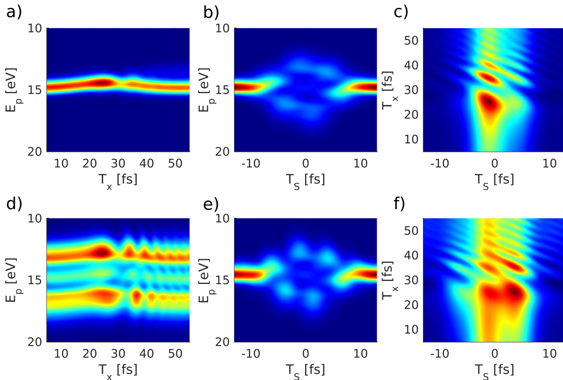
FIG. 5. Streaking spectra for the molecular 1D model with parameters (\sigma_s, \sigma_x) = (8.0, 5.0) fs, (\omega_s, \omega_x) = (0.82, 20) eV. TRPES without (a) and with (d) streaking field ( T_s = 0 ). Photoelectron energy vs. streaking delay for T_x = 7 fs (b) T_x = 35 fs (e). Streaking delay vs. ionization delay for E_p = 12 eV (c) and E_p = 13 eV (f).
