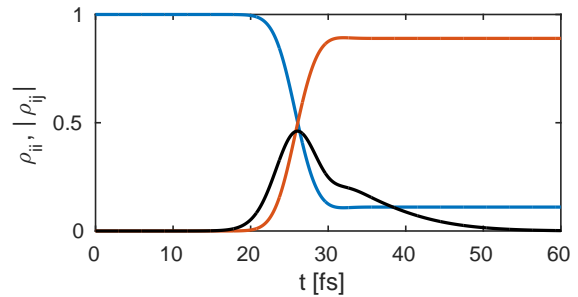
FIG. 4. Time evolution of the electronic populations (state a blue and state b red) for the 1-dimensional molecular model. The magnitude of the electronic coherence ( \rho_{ab} = \langle \phi_a | \phi_b \rangle ) is indicated by the black curve. At \approx 20 fs the molecule hits the avoided crossing.
