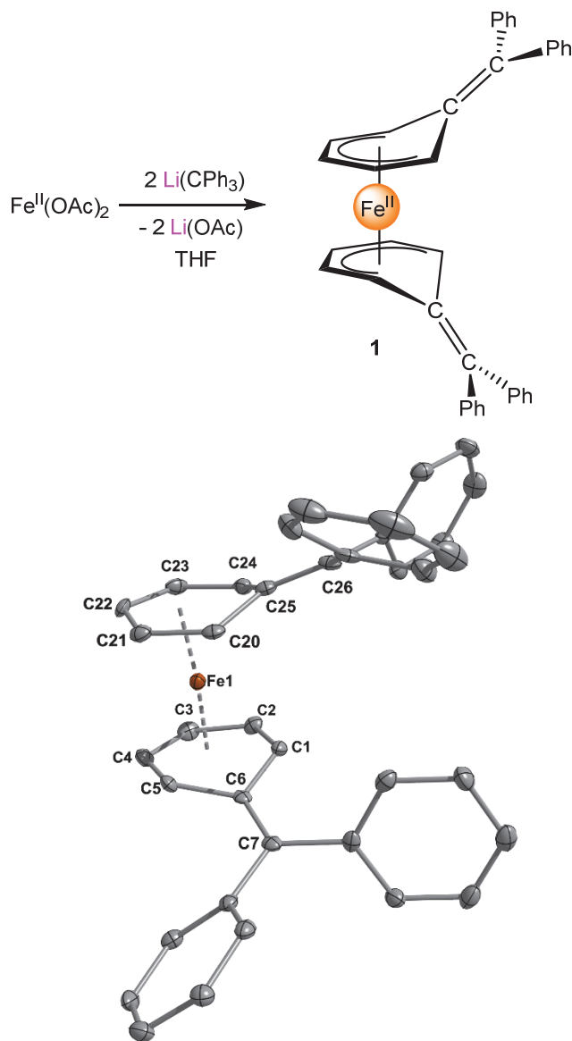
Figure 1. ORTEP drawing of 1 ·CH 2 Cl 2 shown with 50% probability thermal ellipsoids. All hydrogen atoms and methylene chloride solvate are omitted for clarity. Selected bond lengths (Å): Fe1–C1 = 2.121(3), Fe1–C2 = 2.057(3), Fe1–C3 = 2.066(3), Fe1–C4 = 2.047(3), Fe1–C5 = 2.116(3), Fe1–C6 = 2.141(3), Fe1–C21 = 2.056(3), Fe1–C22 = 2.066(3), Fe1–C23 = 2.046(3), Fe1–C24 = 2.112(3), C6–C7 = 1.366(4), C25–C26 = 1.368(4).
