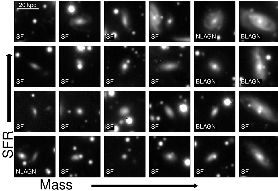
Figure 11. Thumbnails of our H\alpha cluster members. Each square is \sim 40 \times 40 kpc and we organise galaxies in respect to their estimated stellar mass and estimated star-formation rate. We also indicate which sources are likely AGN and which are star-forming. We do not find any evidence for significant galaxy-galaxy (major) merging. This implies that the enhanced star-formation and AGN activity within the merging cluster is not being driven by galaxy-galaxy mergers, and thus is it more likely driven by the interaction with the environment, and in particular with the shock wave. We note that the bright point sources, which show up in most images are stars within the Milky Way, not galaxies.
