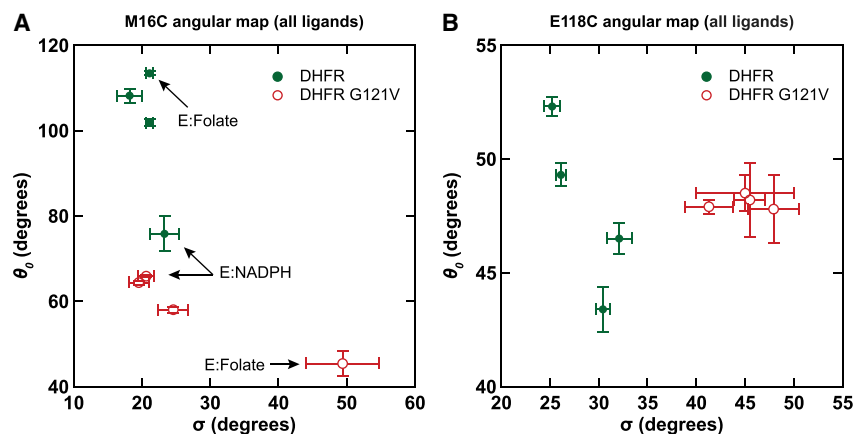
FIGURE 4 DHFR and DHFR-G121V angular maps. Shown are the mean angle and distribution width for apo, NADPH, NADP + , and folate complexes at the M16C (A) and E118C (B) sites for DHFR (green, solid) and DHFR-G121V (red, open). (A) The M16C site exhibits large \theta_0 differences between DHFR and DHFR-G121V. \theta_0 values for DHFR-G121V indicate a conformation distinct from the DHFR closed (E:NADPH) and occluded (E:Folate) states. Error bars represent SD ( n = 10 to 20 replicates). (B) Marked increases in \sigma between DHFR and DHFR-G121V are observed at the E118C site for all ligands, indicating an increase in the flexibility of the F-G loop close to the mutation site. Error bars represent SD ( n = 7 to 20 replicates).
