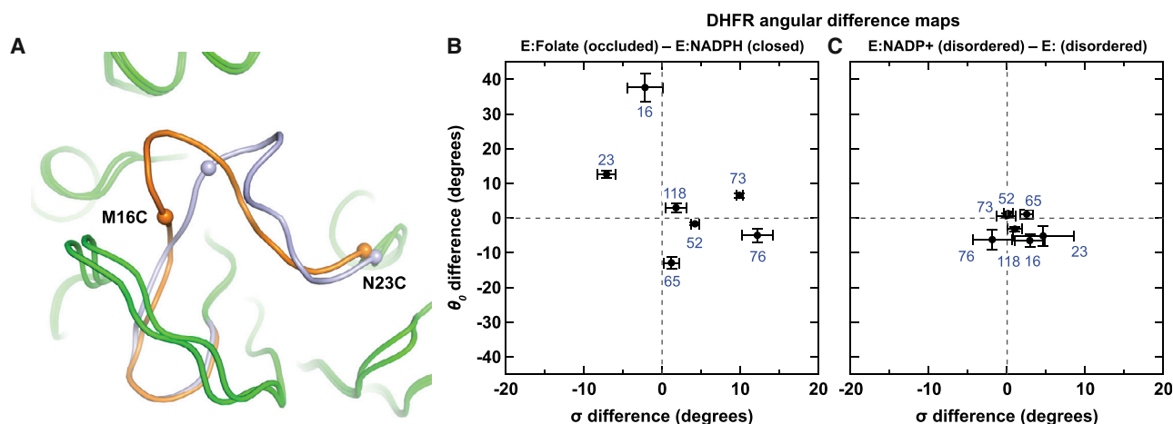
FIGURE 3 Angular differences between DHFR conformational states. (A) X-ray crystal structure overlay highlights the differences in the Met20 loop between the DHFR E:NADPH closed (orange, Protein Data Bank: 1RX1) and the DHFR E:Folate occluded states (blue, Protein Data Bank: 1RX7). (B) Shown is an angular difference map for DHFR E:Folate – E:NADPH (occluded – closed) at all the sites studied. Error bars represent SD ( n = 10 to 20 replicates). (C) Shown is an angular difference map for the DHFR E:NADP+ (disordered) – E: (disordered) states. Error bars represent SD ( n = 7 to 28 replicates).
