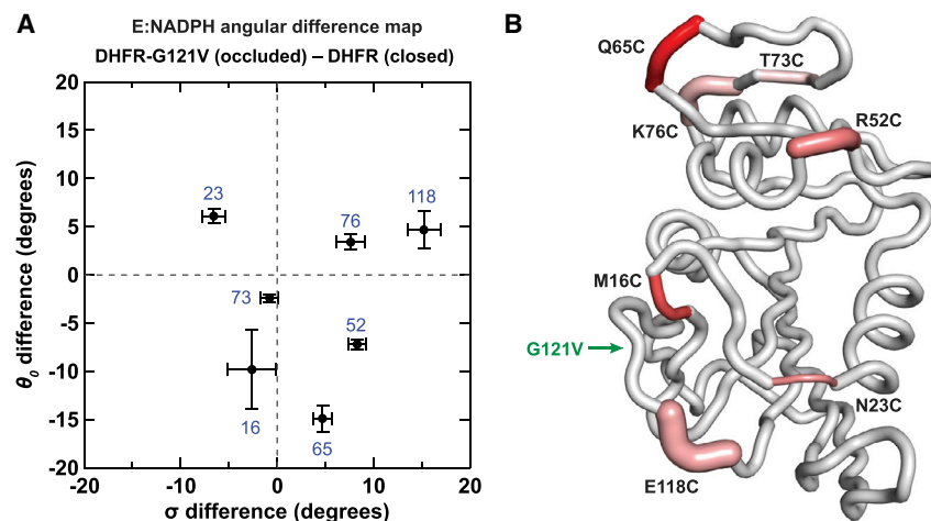
FIGURE 5 DHFR and DHFR-G121V angular differences and model. (A) Shown is an angular difference map between DHFR and DHFR-G121V for the E:NADPH holoenzyme. Pronounced differences occur at the M16C, Q65C, and E118C sites. Error bars represent SD ( n = 9 –20 replicates). (B) Shown is the tube representation of the data in (A) in which relative tube thickness represents \sigma differences, and darker shades of red indicate larger absolute \theta_0 differences. The angular model is overlaid on the DHFR E:NADPH structure (Protein Data Bank: 1RX1), and highlighted areas include the probe sites and immediately adjacent residues. The G121V mutation site is indicated by a green arrow.
