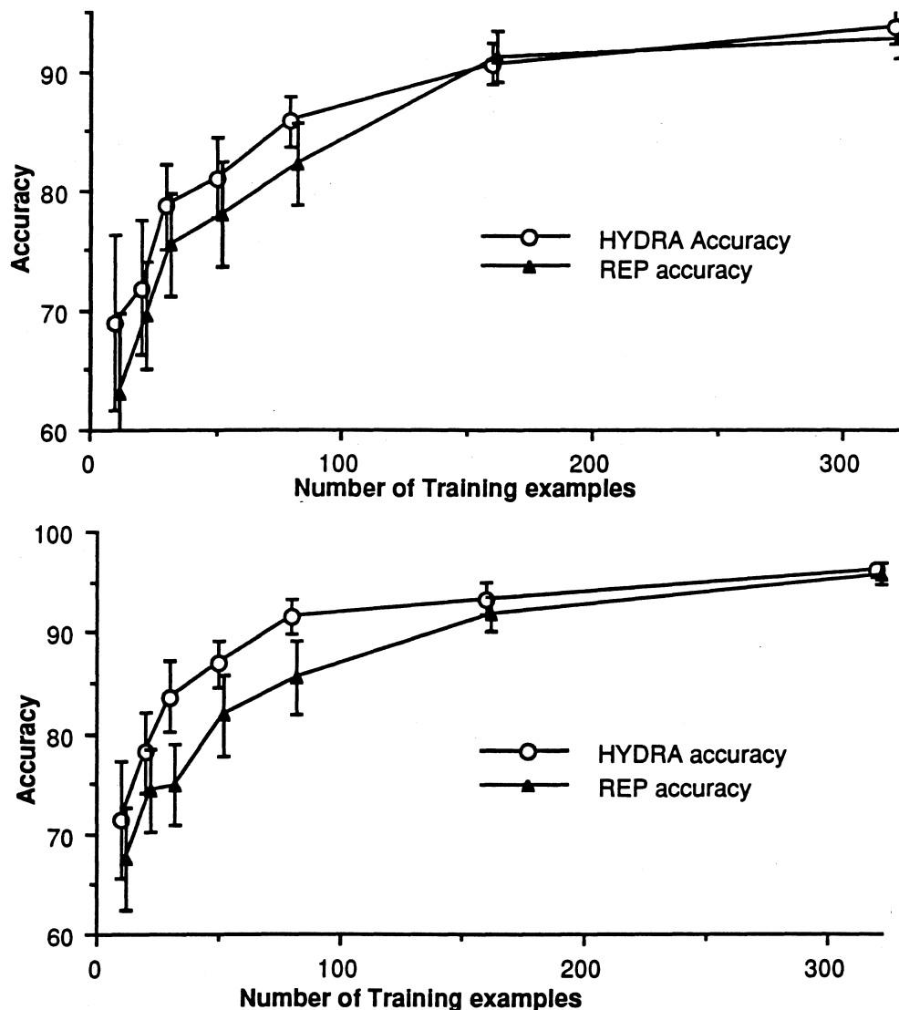
Figures 3a and 3b. Comparison of HYDRA and REP on KRK with 20% class noise and 5% tuple noise, respectively. Standard-deviation bars are shown.
