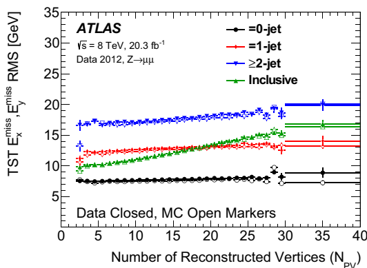
Fig. 8 The resolution of the combined distribution of E_T^{\text{miss}} and E_V^{\text{miss}} for the TST E_T^{\text{miss}} as a function of N_{PV} for the 0-jet, 1-jet, \geq 2 -jet, and inclusive Z \rightarrow \mu\mu samples. The data (closed markers) and MC simulation (open markers) are overlaid. The jet counting uses the same JVF criterion as the TST E_T^{\text{miss}} reconstruction algorithm
