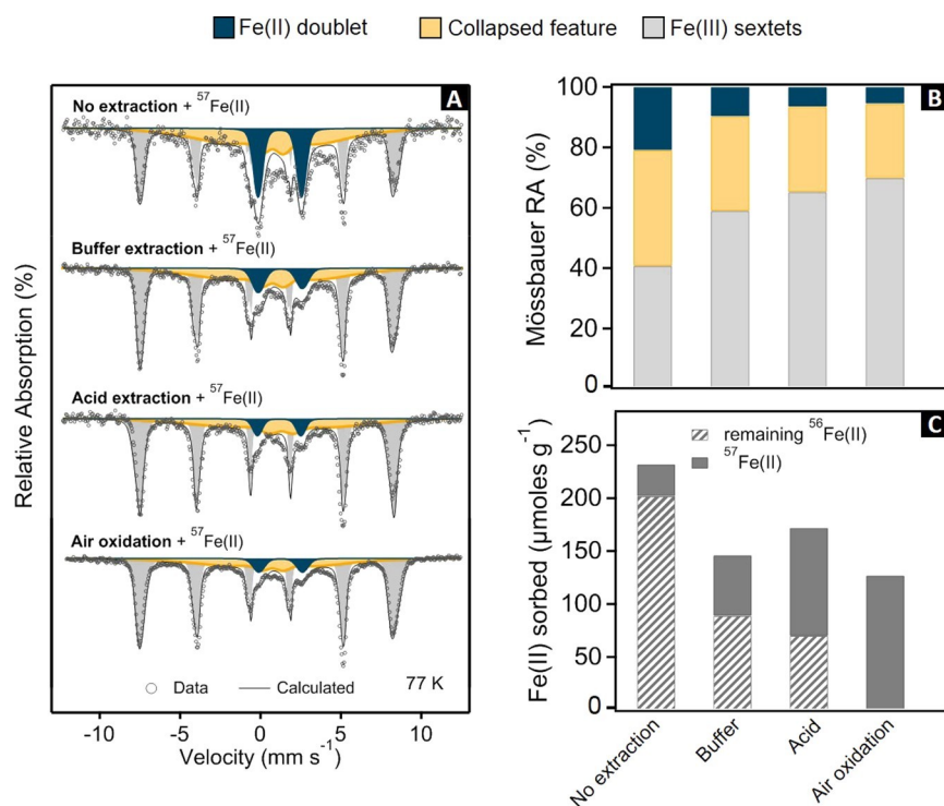
Figure 4. (A) Mössbauer spectra of ^{56}\text{goethite} reacted with 1\text{ mM } ^{57}\text{Fe(II)} after previous reaction with 1\text{ mM } ^{56}\text{Fe(II)} [1 month], before and after buffer extraction, acid extraction, and air oxidation. (B) Relative Mössbauer spectral area (RA) of Fe(III) sextets, Fe(II) doublet, and collapsed feature for panel A samples. (C) Amount of ^{56}\text{Fe(II)} and ^{57}\text{Fe(II)} sorbed for samples in panel A.
