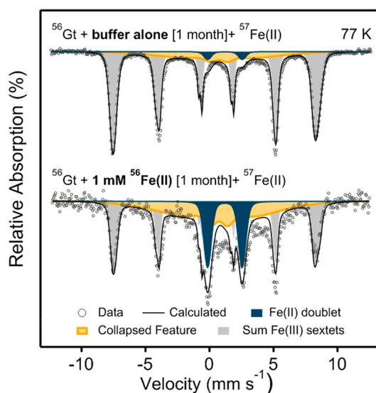
Figure 1. Mössbauer spectra of ^{56}\text{Fe} goethite aged for one month in buffer alone and reacted with 1 mM ^{57}\text{Fe(II)} (top spectrum). ^{56}\text{Fe} goethite aged in 1 mM ^{56}\text{Fe(II)} for one month and reacted with 1 mM ^{57}\text{Fe(II)} (bottom spectrum).
