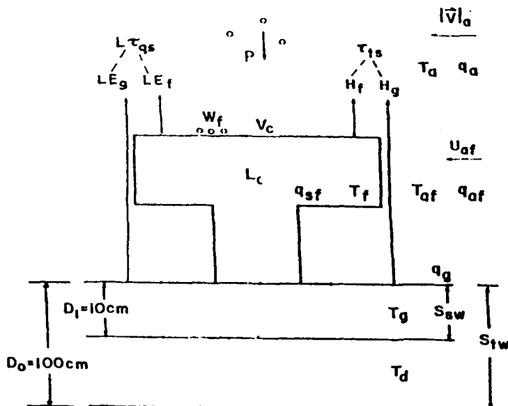
Fig.1. A schematic diagram denoting the components of the surface hydrological cycle. V_c is the vegetation cover, P the precipitation, T_a , T_{af} , T_f , T_g , and T_d the temperatures above the vegetation layer, within the foliage layer, of the foliage, at the surface soil, and subsurface, respectively, q_a and q_{af} the mixing ratios above and within the vegetation layer, respectively, q_{sf} and q_g the saturated mixing ratios at temperatures T_f and T_g , respectively, S_{sw} the surface soil water in the upper layer of soil, S_{tw} the total water in the rooting zone of soil, E_g and E_f fluxes of water vapor from the ground and foliage, respectively, H_g and H_f the sensible heat fluxes from the ground and foliage, respectively, L_c the leaf area index.
