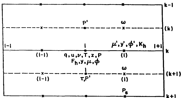
Fig.2. Grid points used in the two-dimensional model (see text for further explanation).
