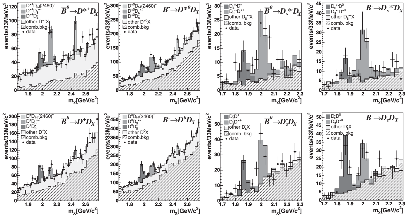
FIG. 2. Distributions of m_X . Fitted \bar{B} \rightarrow D^{(*)+,0} D_s^{(*)-} and \bar{B} \rightarrow D^{(*)+,0} D_{sJ}(2460)^- signal contributions and background components, determined as described in the text, are overlaid to the data points.
