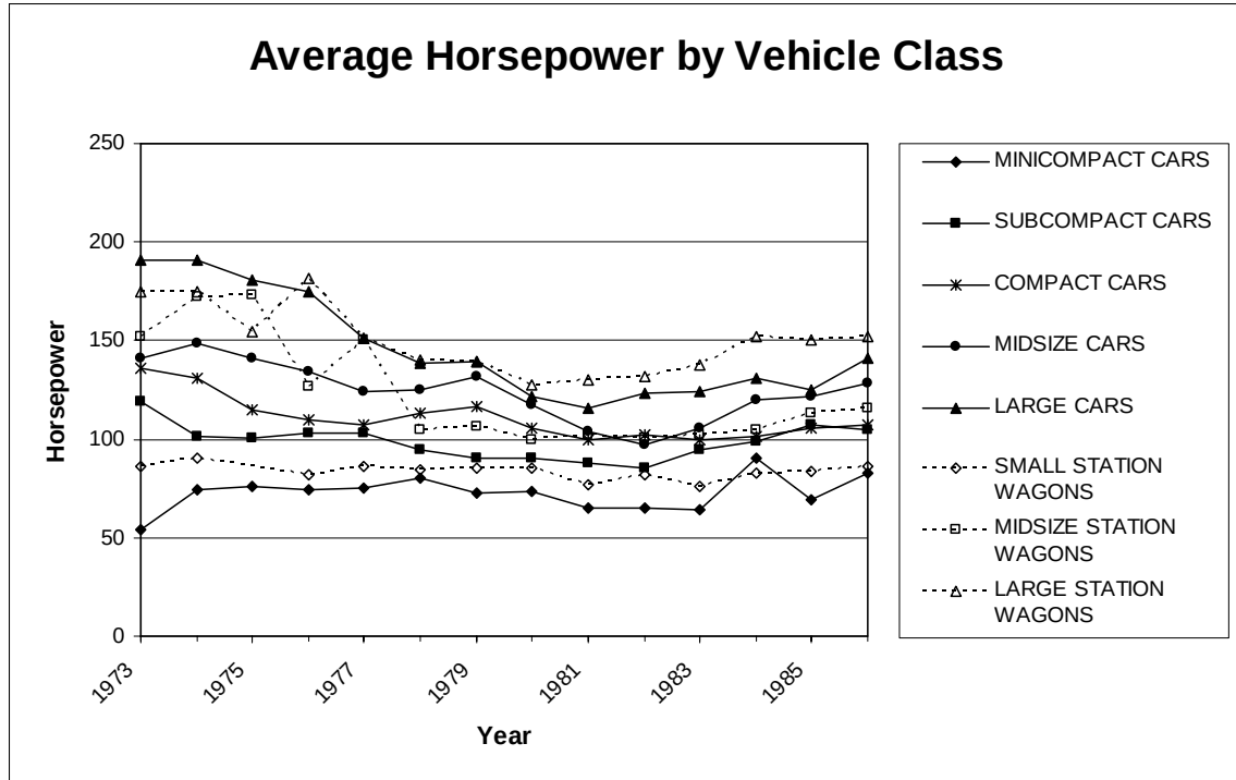
Figure 2.3 Average Horsepower by Vehicle Class
