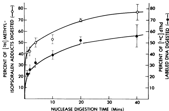
FIGURE 3. Percentage of [ ^3\text{H} ]5-MIP adducts (○) and [ ^{14}\text{C} ]labeled DNA (●) rendered soluble by micrococcal nuclease as a function of digestion time using nuclei prepared from XP12RO cells.
