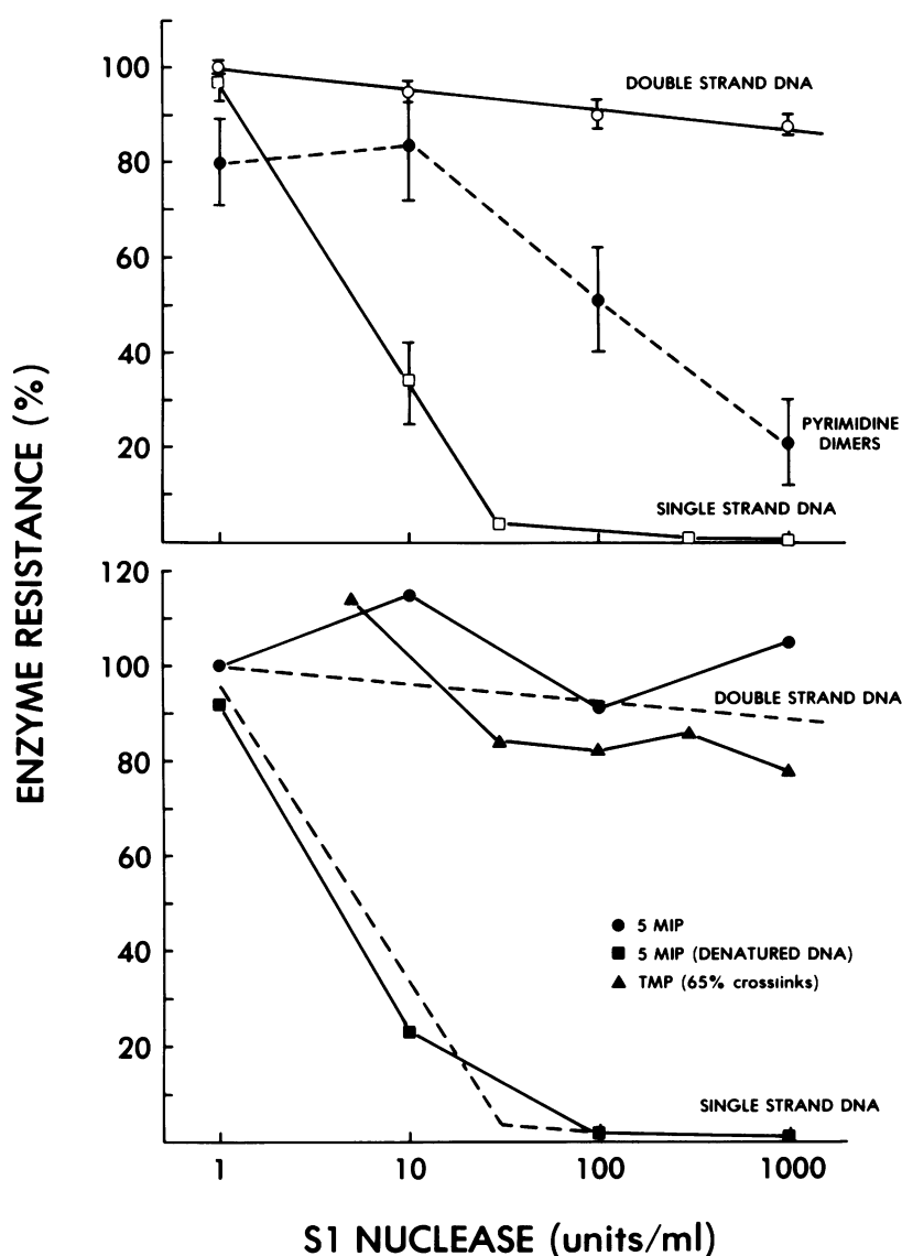
FIGURE 2. Acid-soluble nucleotides released from purified DNA incubated with various concentrations of S1 nuclease (37°C, 30 min): (top) (○) ^{14}\text{C} -labeled double-stranded DNA; (□) ^{14}\text{C} -labeled single-stranded DNA; (●) cyclobutane pyrimidine dimers; (bottom) (●) [ ^3\text{H} ]5-MIP-labeled DNA; (■) [ ^3\text{H} ]5-MIP-labeled DNA denatured by boiling for 10 min and quenching in ice; (▲) [ ^3\text{H} ]trimethylpsoralen (crosslink frequency determined by heat denaturation followed by S1 nuclease digestion).
