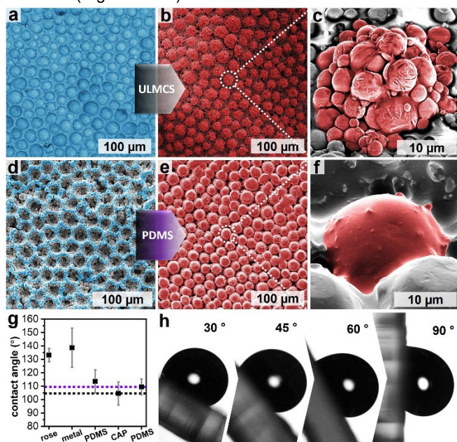
Figure 4. Process of creating a metallic and PDMS rose replica. a) Inverse PDMS rose as the template for creating metallic b) rose replica and c) associated zoom-in. d) inverse metal rose pattern used as a mold for PDMS, f) fabricated PDMS male rose patterns. f) zoom-in feature. g) Static contact angle formed by water droplets on formed surfaces. Difference between analogous structures on rose, metal, and PDMS, referenced to non-patterned PDMS (marked with top dotted line) and chemical activated ULMCS (marked with bottom dotted line). h) droplet shape variation on metal rose surface when the surface is tilted to 30, 45, 60 and 90 degrees.
