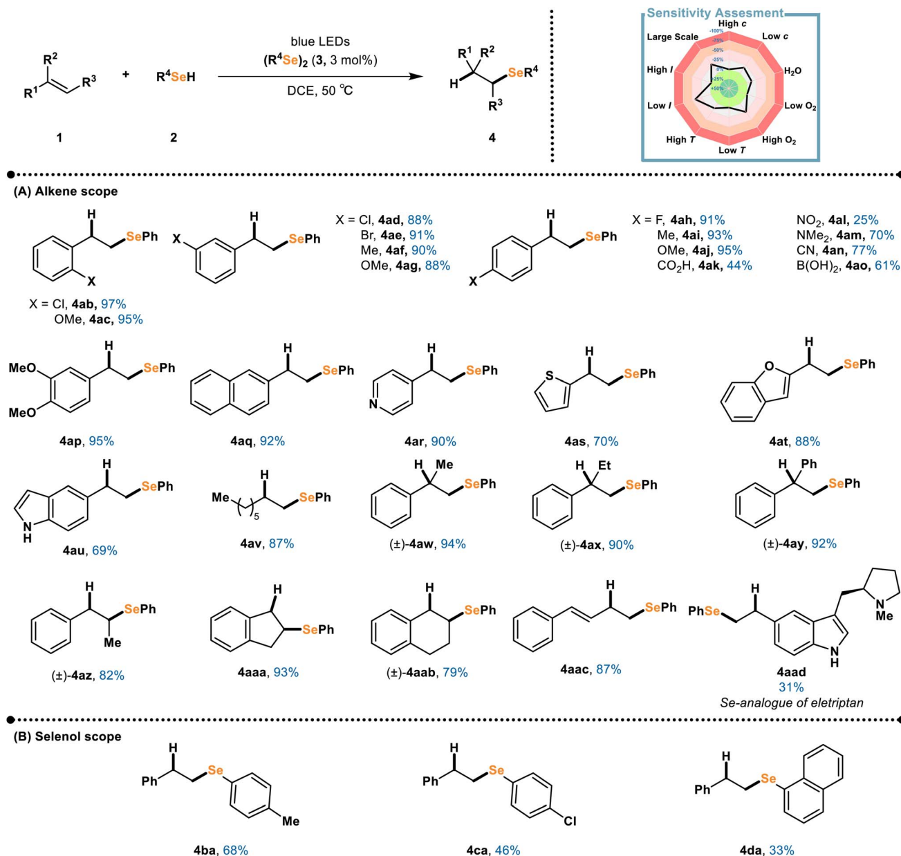
Fig. 2 Scope of light-catalyzed hydroselelenation for (A) alkenes and (B) selenols. Reaction conditions for alkene scope: 1 (1.0 equiv.), 2 (1.5 equiv.), 1,2-dichloroethane (0.25 M). Reaction conditions for selenol scope: 1 (1.0 equiv.), 3 (1.5 equiv.), Ph 2 POH (1.5 equiv.), 1,2-dichloroethane (0.25 M). Reactions are run in a light box under blue LEDs and monitored by TLC for reaction completion (20 min to 24 h). Temperature in the box rises to 50 °C in 20 minutes due to LEDs and maintains that temperature over time. Regioselectivity determined by 1 H NMR analysis of the unpurified reaction mixture.
