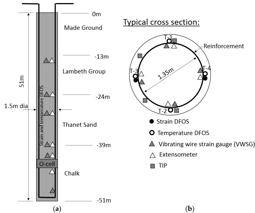
Figure 2. Geometry and instrumentation of the test pile: (a) plan view; (b) cross-section.
