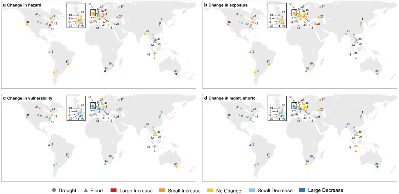
Extended Data Fig.1 | Location of flood and drought paired events coloured according to their indicators-of-change. a, Change in hazard; b, change in exposure; c, change in vulnerability and d, change in management shortcomings.
