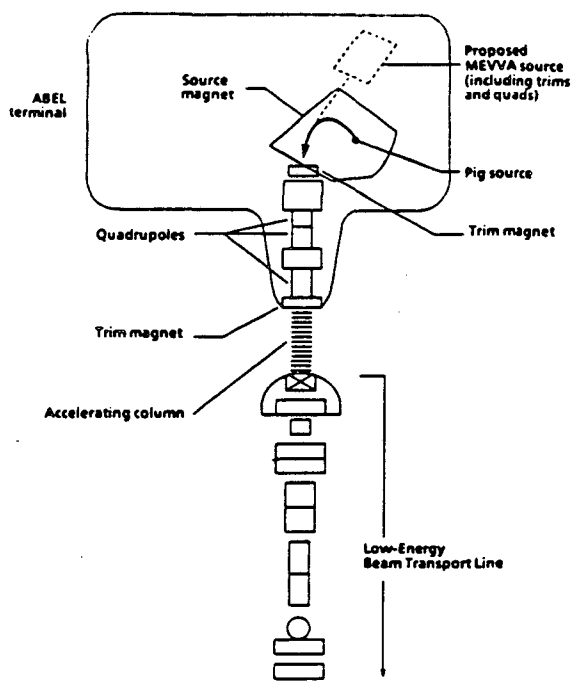
ABEL injector, showing proposed MEVVA source
