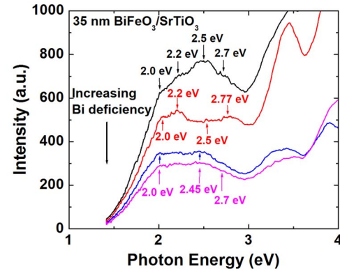
FIG. 3. (Color online) CL spectra measured at a beam voltage of 1 kV (corresponding to a penetration depth of 18 nm) for Bi-deficient BiFeO 3 films grown by MBE.
