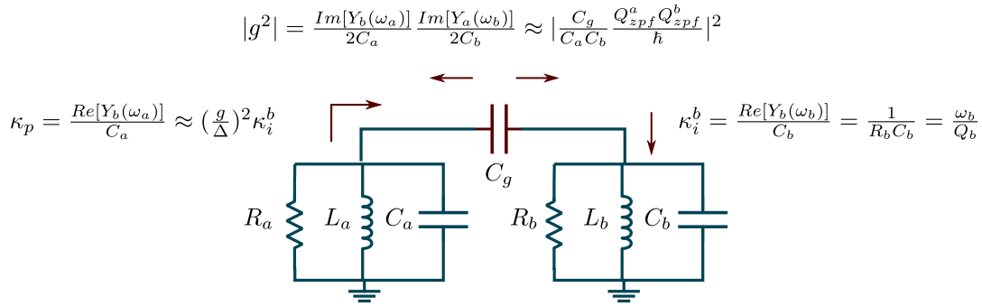
Figure 2.3: Capacitive coupling of two dissipative LC resonators.
