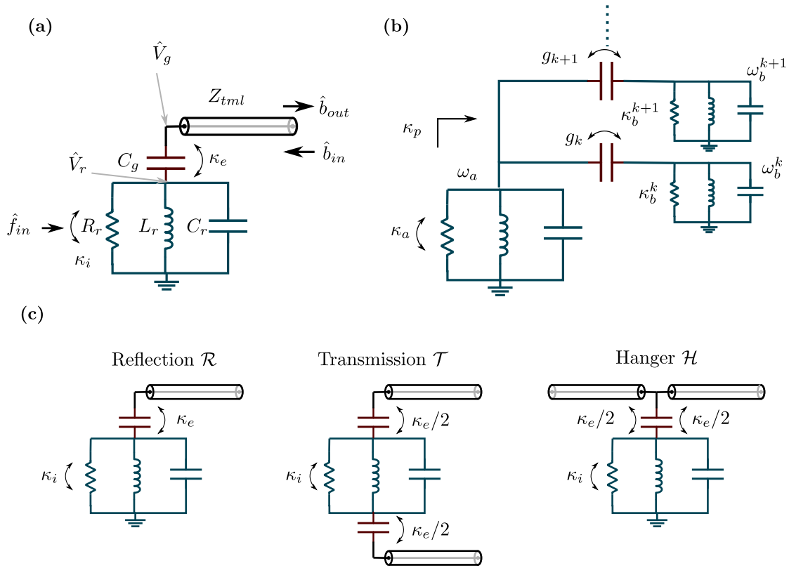
Figure 2.6: Harmonic oscillator coupled to dissipative environments: (a) infinite-length transmission line, (b) a bosonic bath of damped resonators, and (c) coupling configurations.
