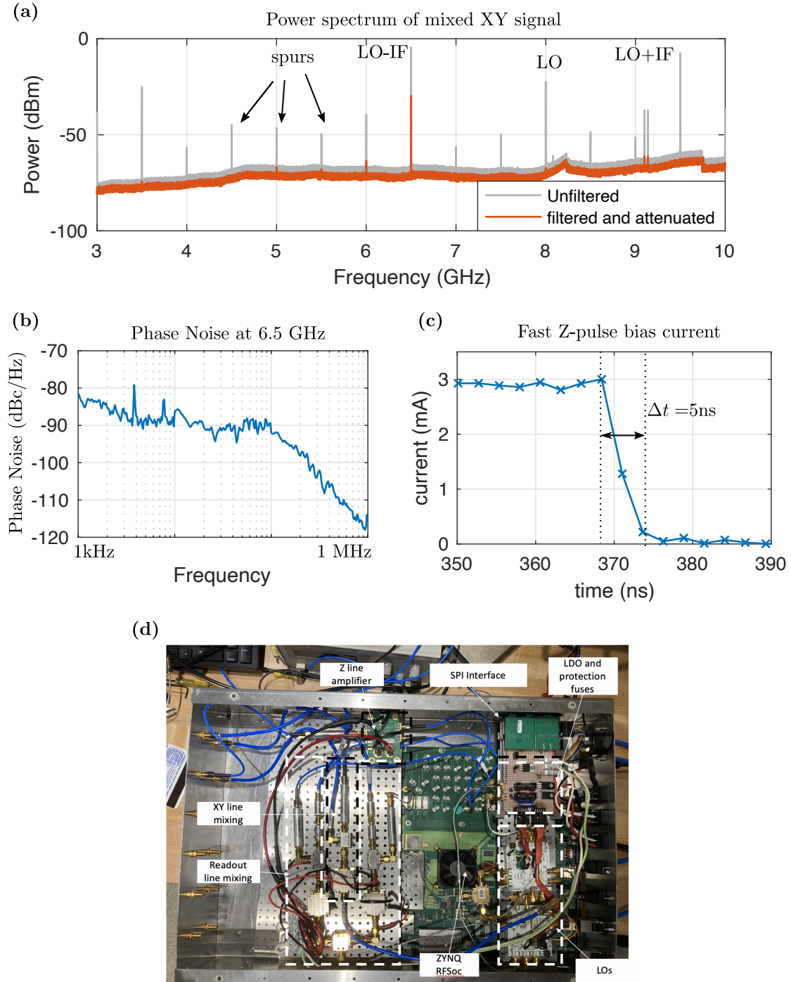
Figure 4.6: Room Temperature microwave characterization: (a) power spectrum scan of the XY line with and without filters, (b) local oscillator phase noise, (c) Z-line rise/fall time, and (d) image of the assembled FPGA measurement hardware.
