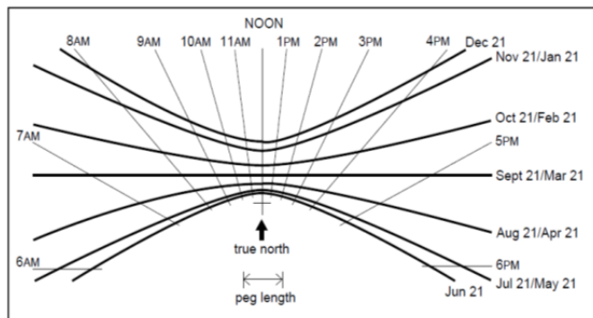
Figure 27: Sizing of fins and overhangs
