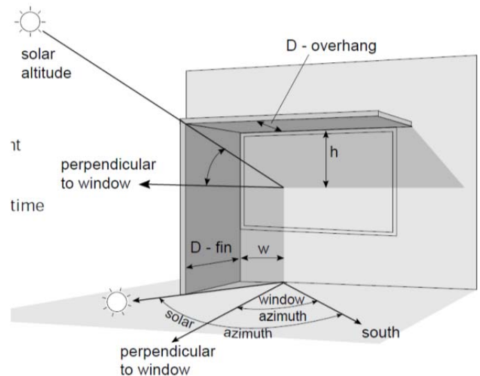
Figure 27: Sizing of fins and overhangs
